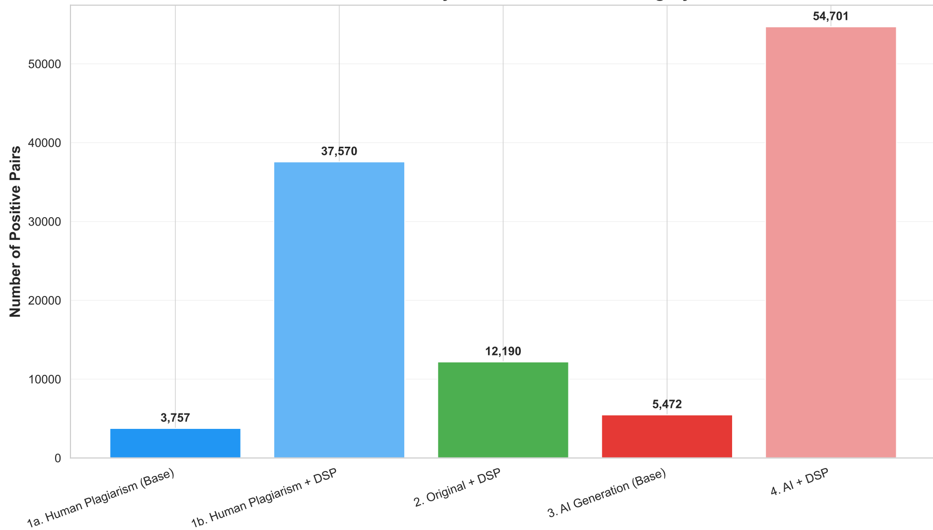
Positive Pairs by Broad Modification Category
