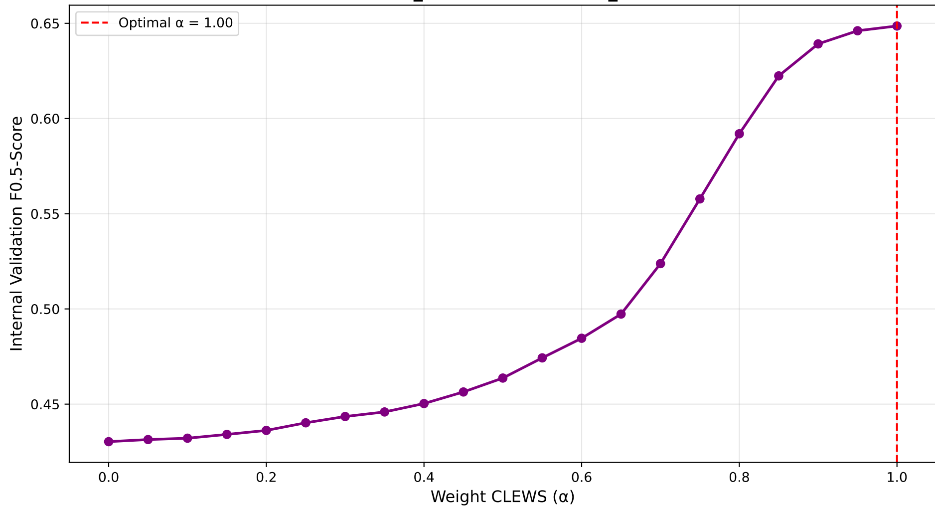
F0.5-Score vs Alpha (manhattan_distance & cosine_distance)
