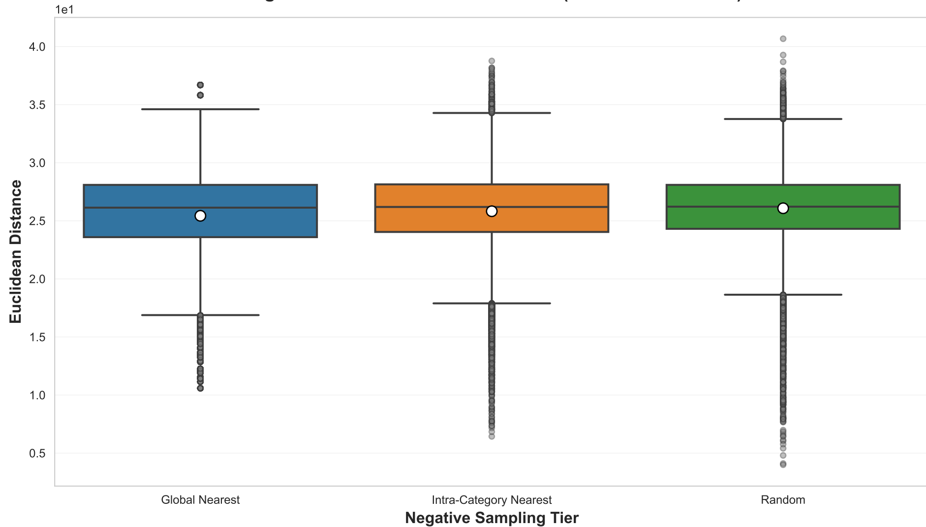
Negative Tier Distribution — WEALY (Euclidean Distance)
