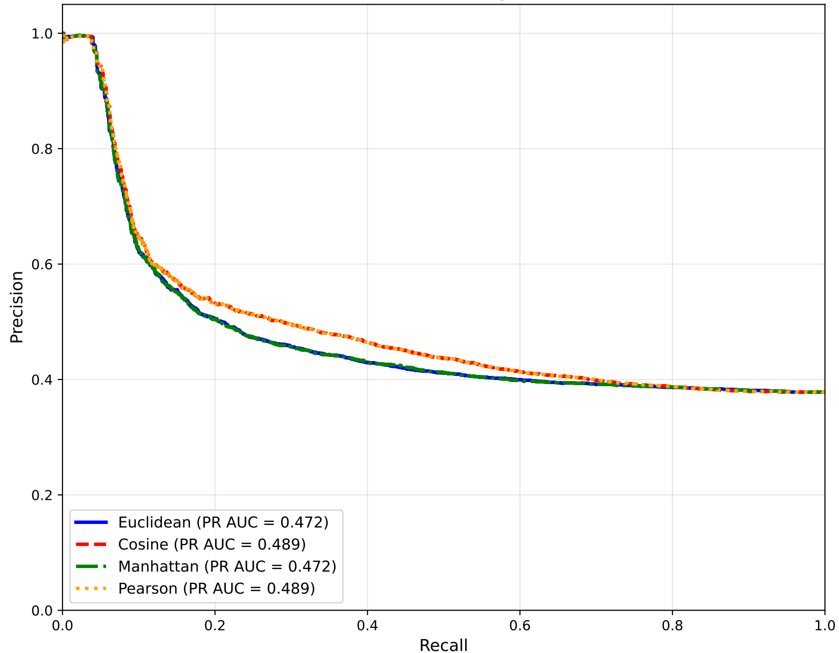
Precision-Recall Curve Comparison — WEALY
