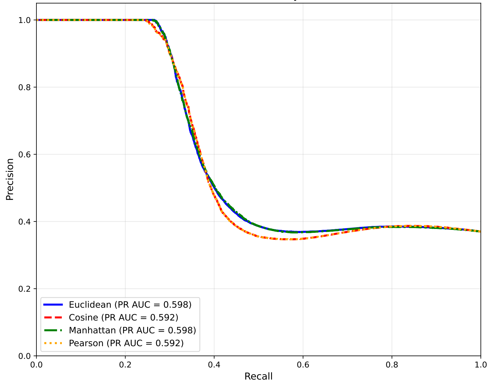
Precision-Recall Curve Comparison - CLEWS
