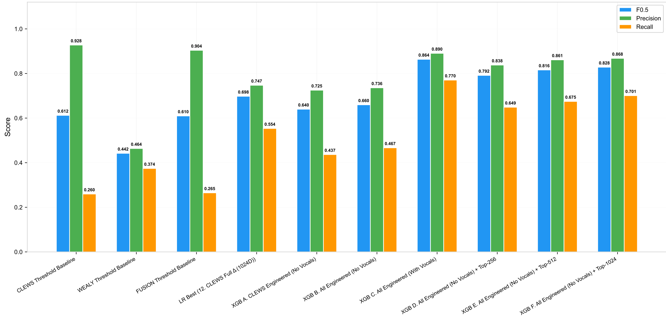
XGBoost Convergence Study: Engineered + Top-K Actual Dimensions
