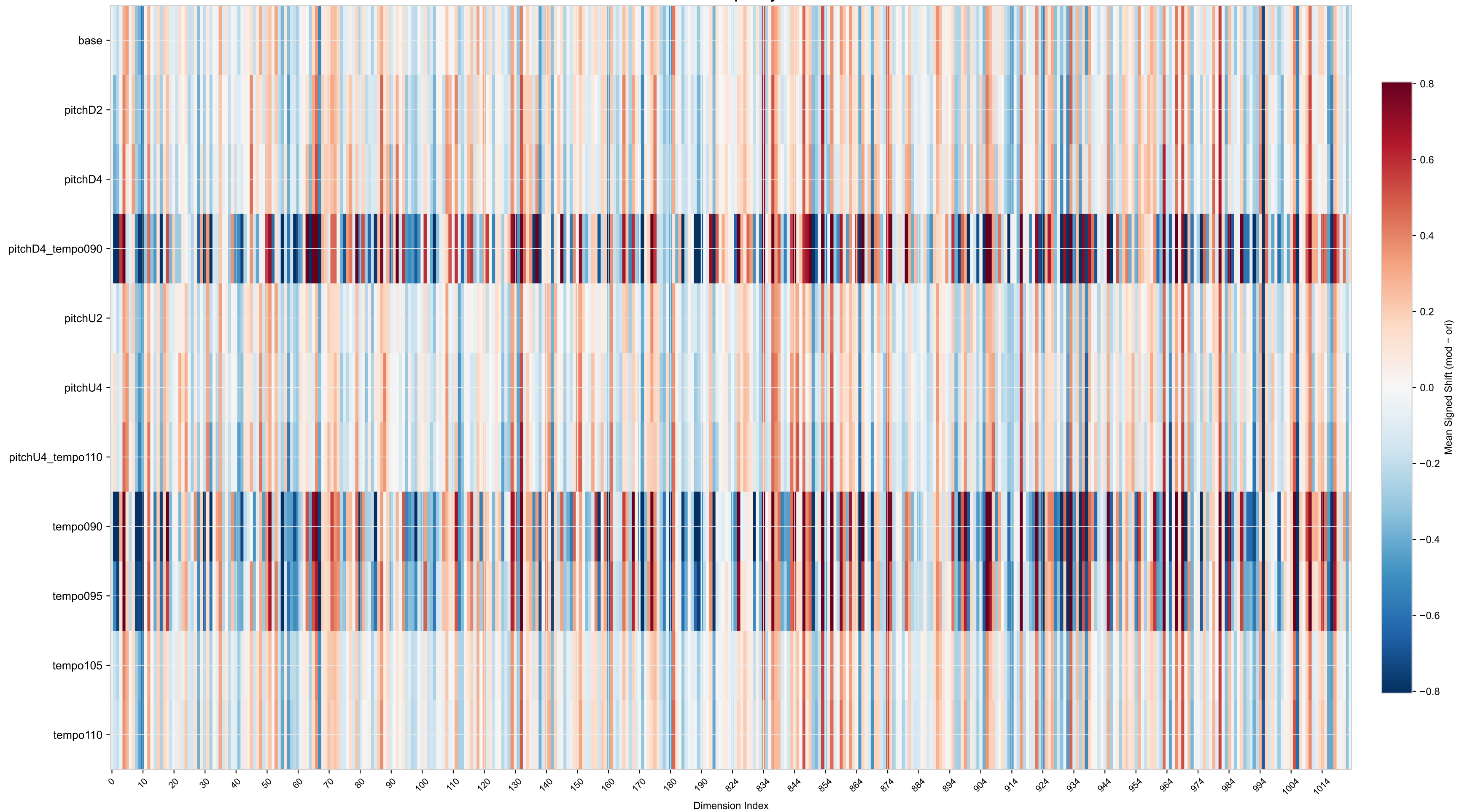
CLEWS — Signed Mean Shift per Dimension (first 200 + last 200 of 1024 dims) All sources · Grouped by: DSP Label
