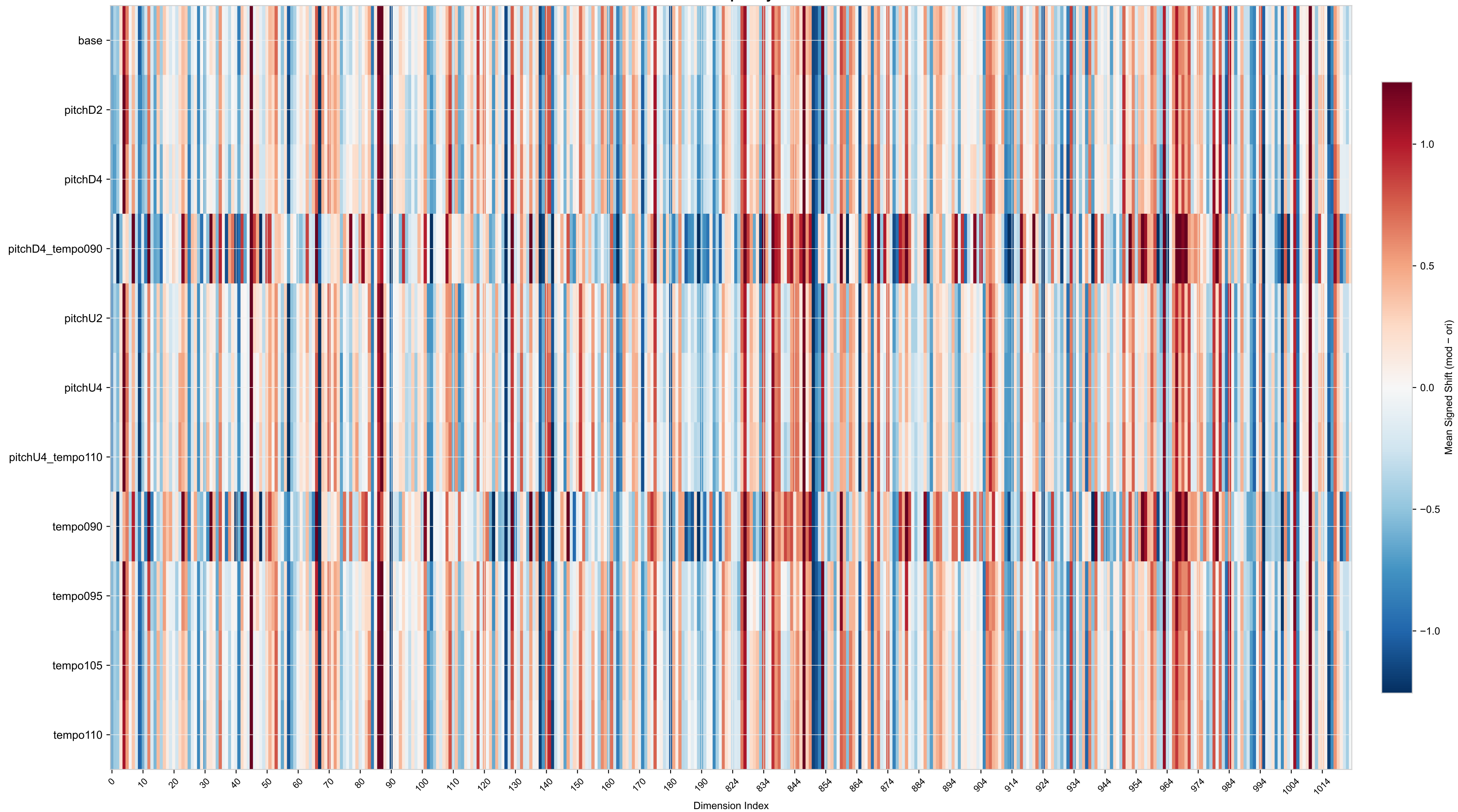
CLEWS — Signed Mean Shift per Dimension (first 200 + last 200 of 1024 dims) MusicGen · Grouped by: DSP Label
