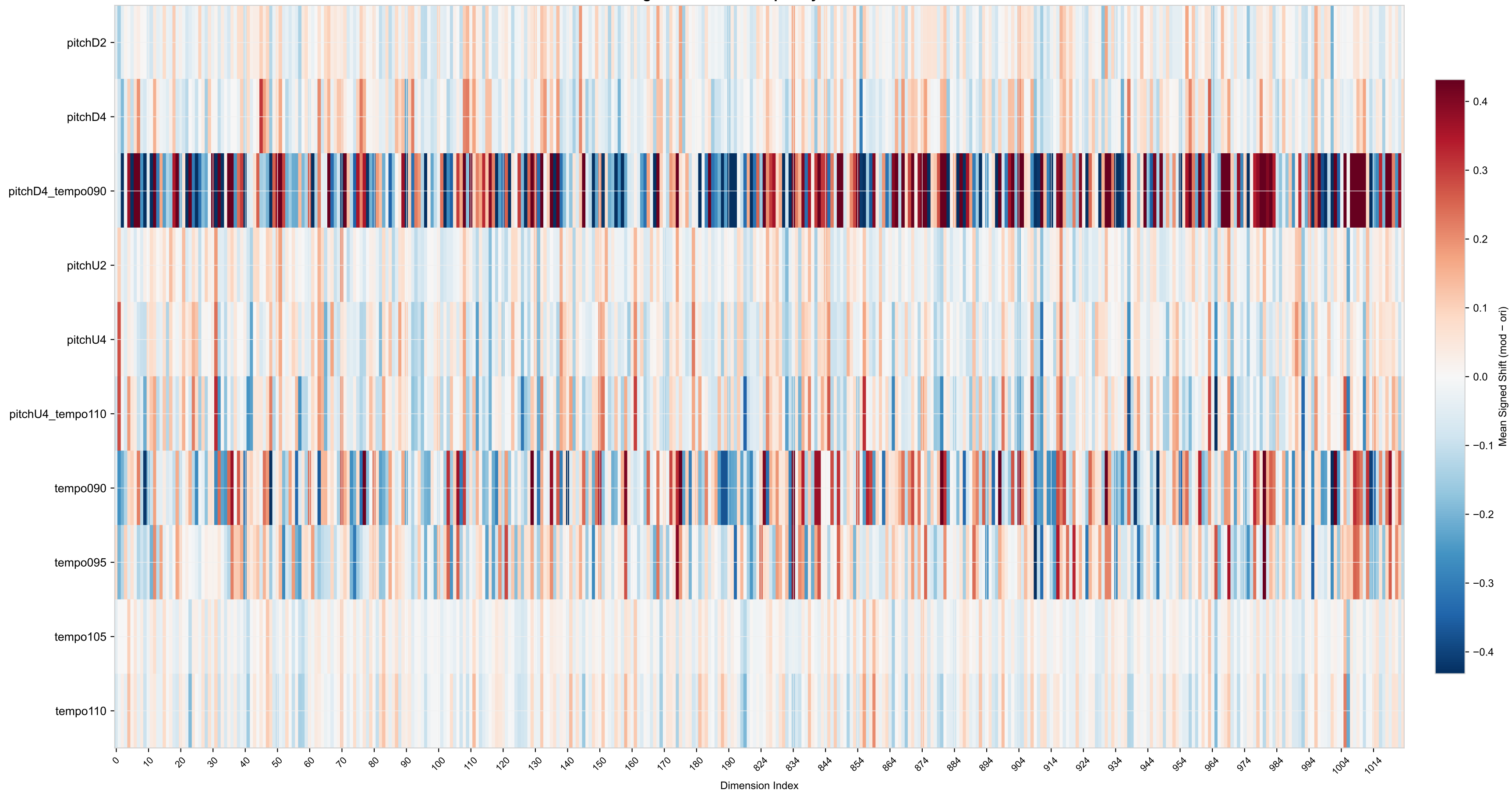
CLEWS — Signed Mean Shift per Dimension (first 200 + last 200 of 1024 dims) Original + DSP · Grouped by: DSP Label
