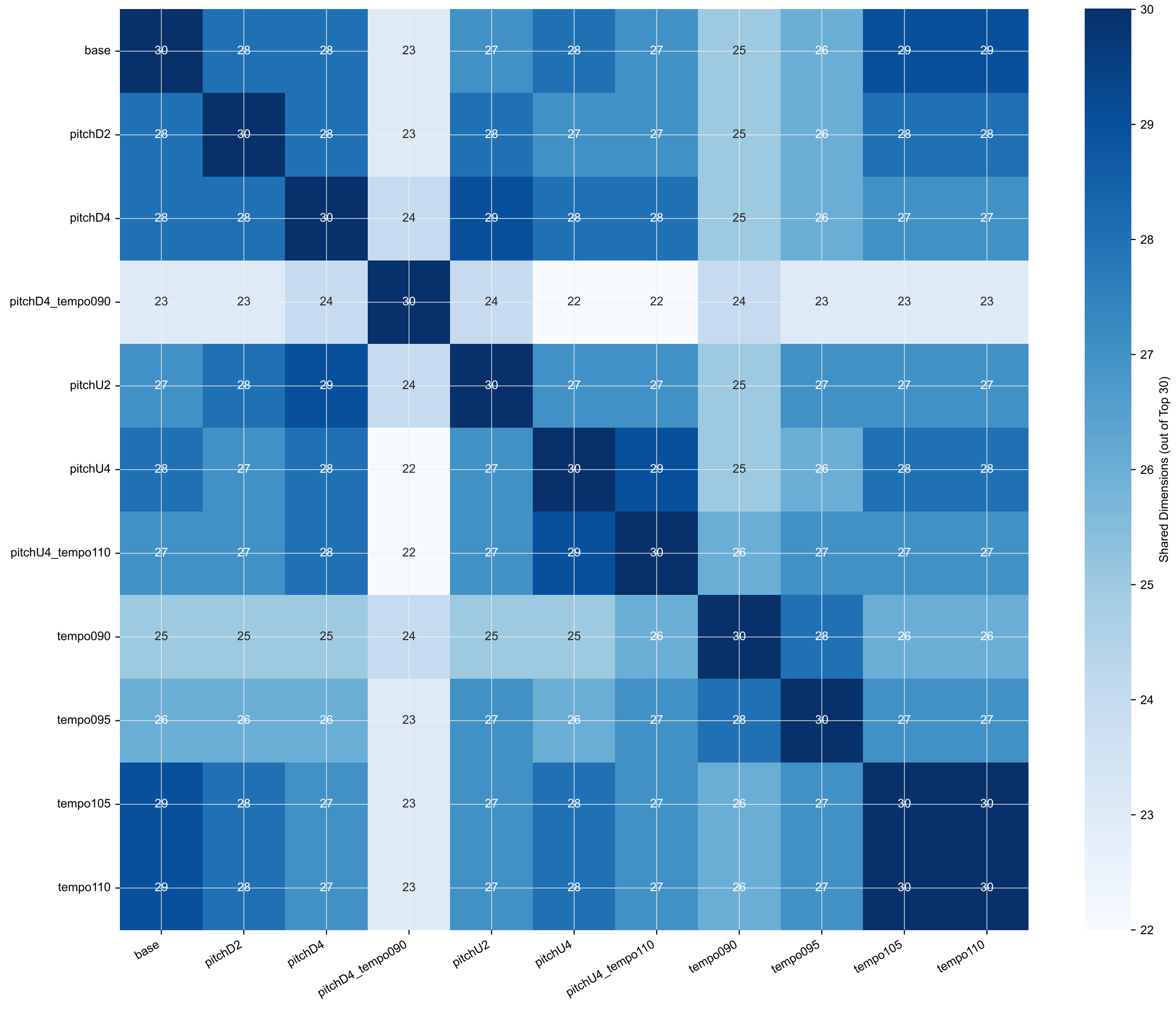
CLEWS — Top-30 Dimension Overlap Between Categories All sources · Grouped by: DSP Label
