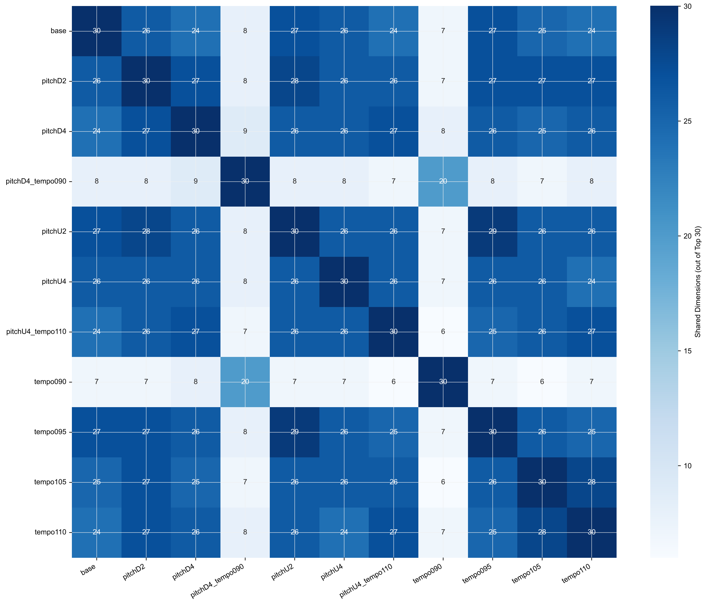
CLEWS — Top-30 Dimension Overlap Between Categories MGE-LDM Drums · Grouped by: DSP Label
