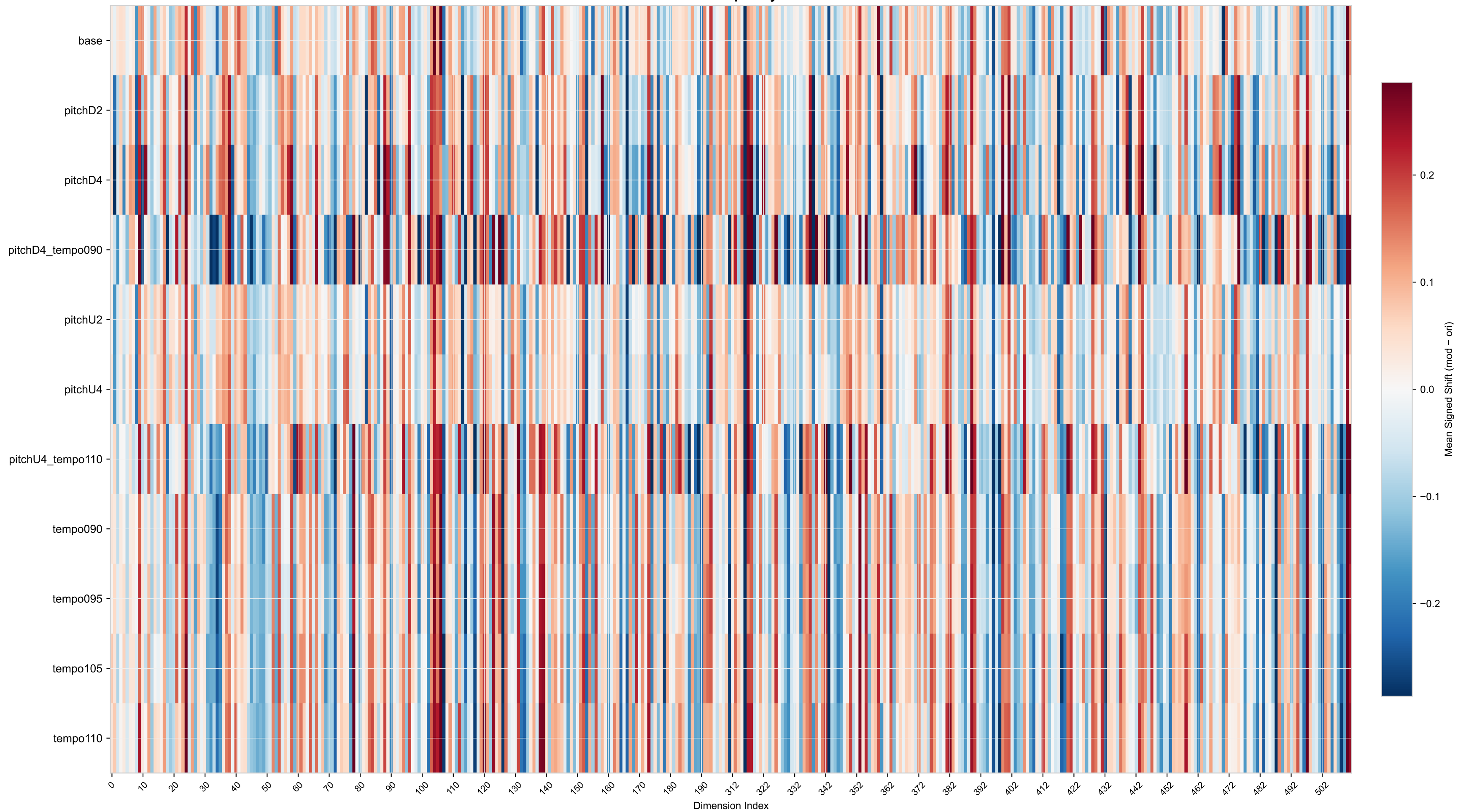
WEALY — Signed Mean Shift per Dimension (first 200 + last 200 of 512 dims) All sources · Grouped by: DSP Label
