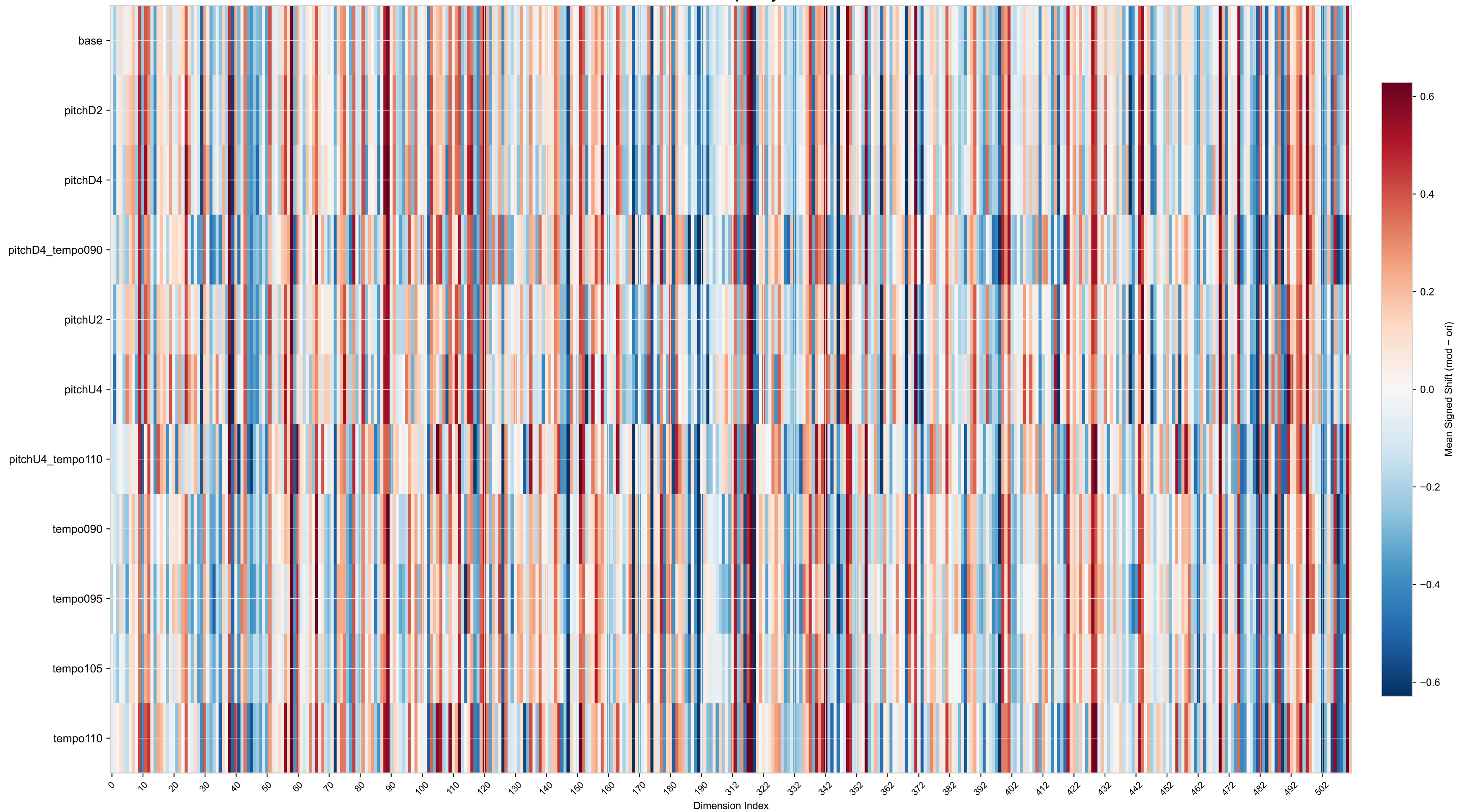
WEALY — Signed Mean Shift per Dimension (first 200 + last 200 of 512 dims) AudioLDM2 · Grouped by: DSP Label
