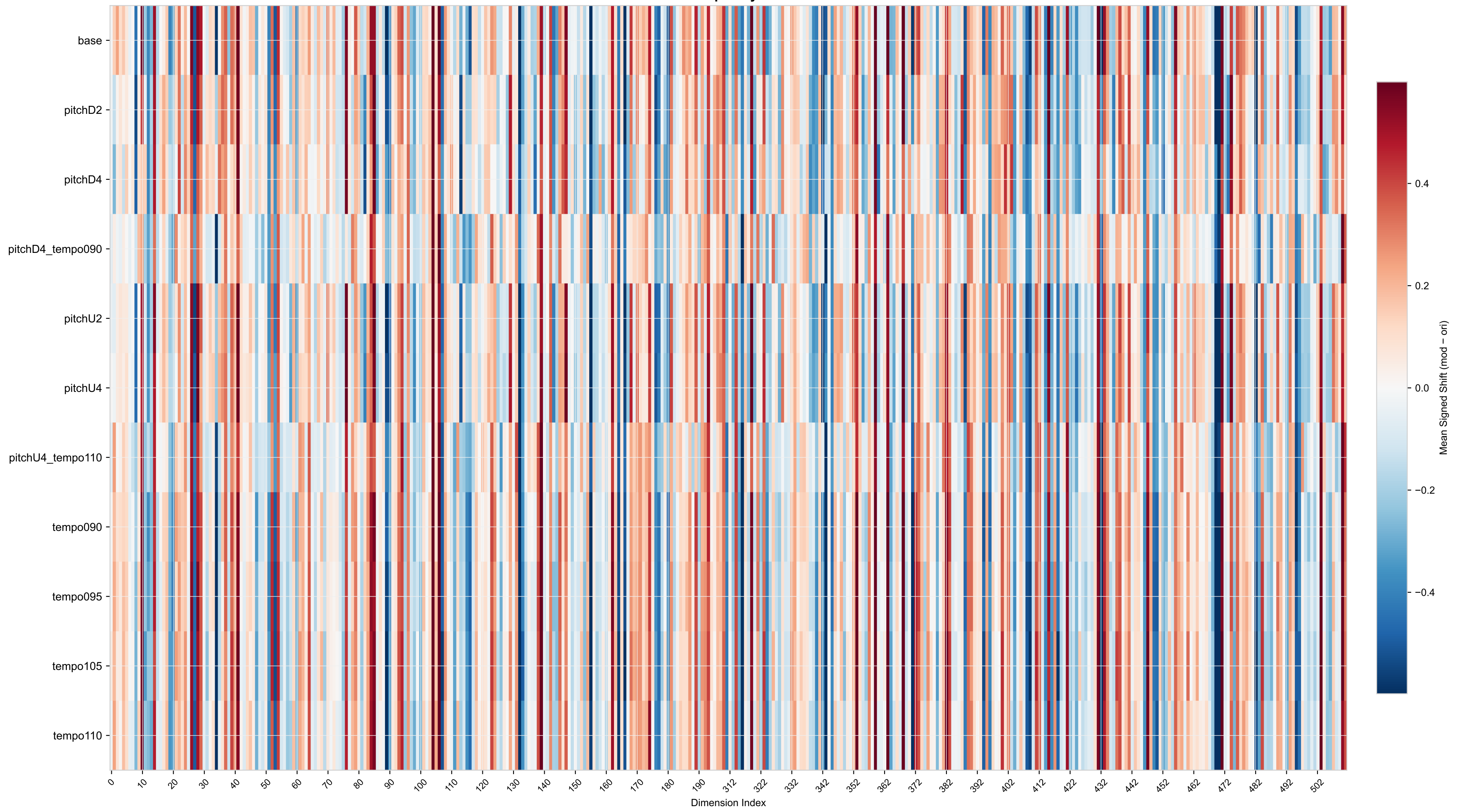
WEALY — Signed Mean Shift per Dimension (first 200 + last 200 of 512 dims) Cover · Grouped by: DSP Label
