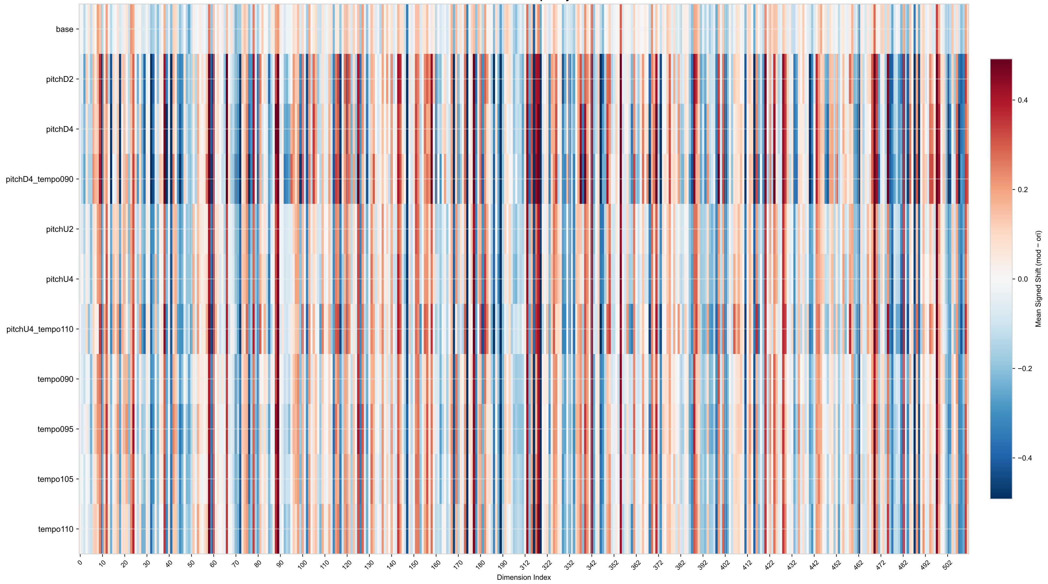
WEALY — Signed Mean Shift per Dimension (first 200 + last 200 of 512 dims) MGE-LDM Drums · Grouped by: DSP Label
