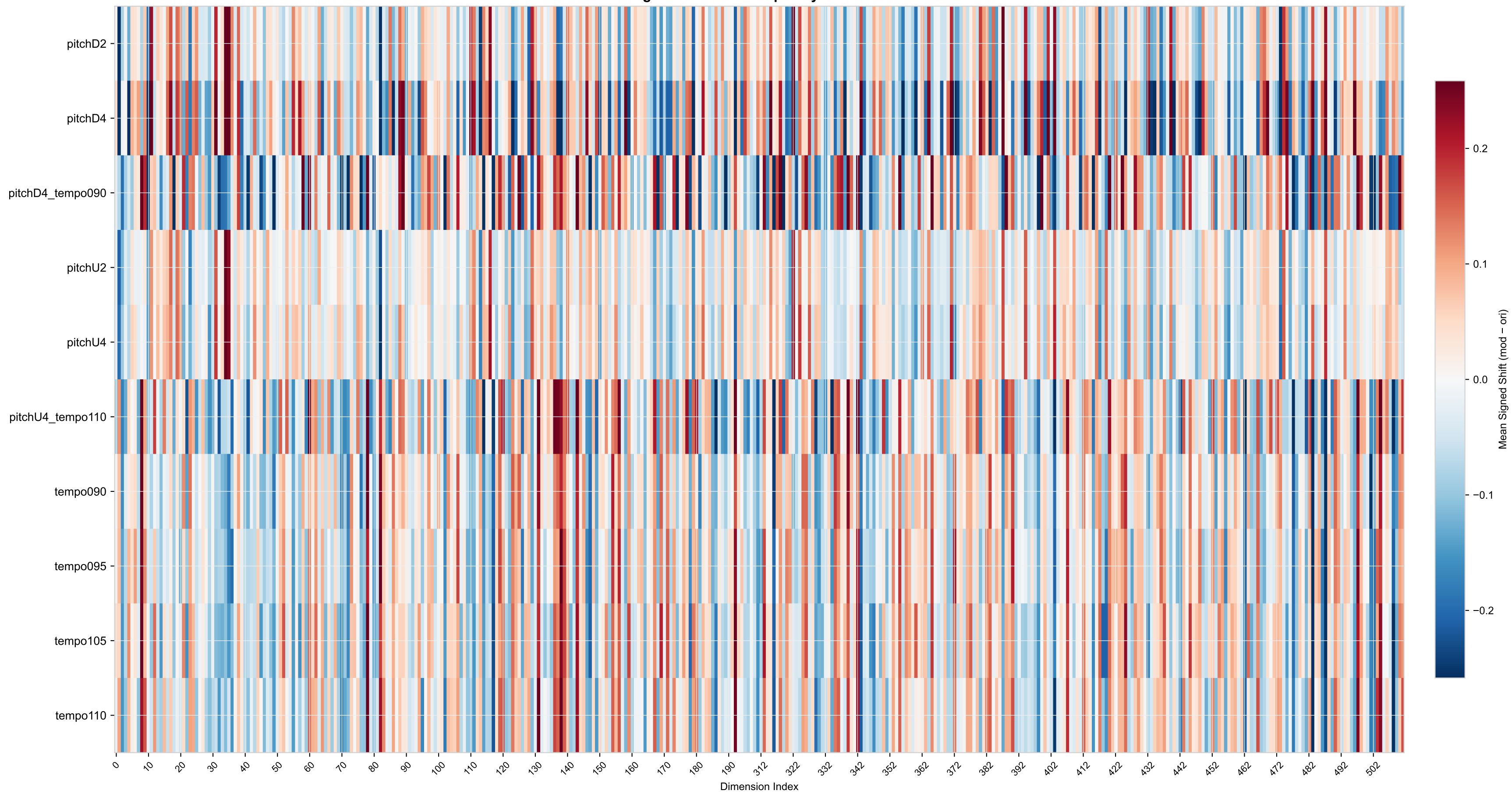
WEALY — Signed Mean Shift per Dimension (first 200 + last 200 of 512 dims) Original + DSP · Grouped by: DSP Label
