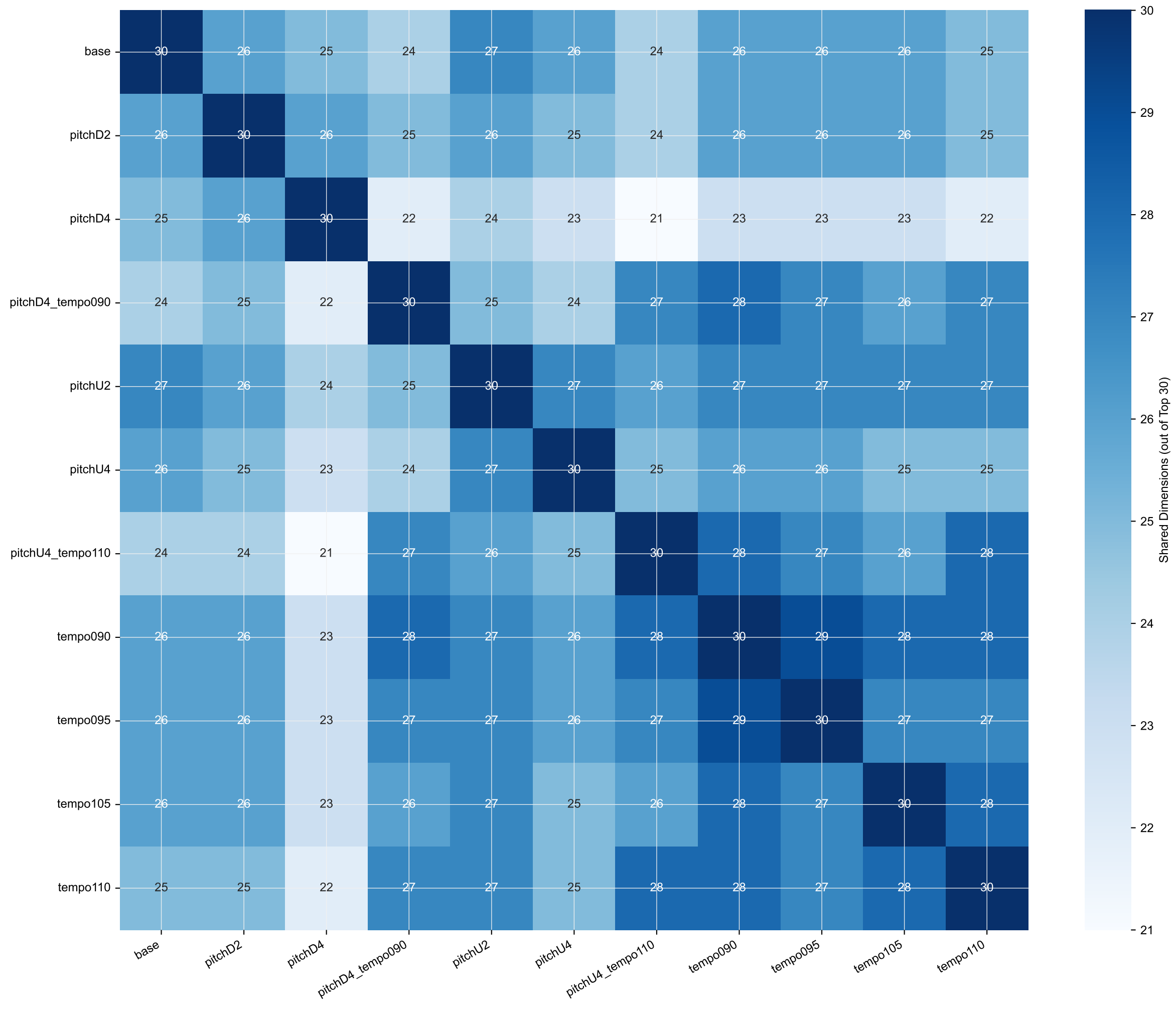
WEALY — Top-30 Dimension Overlap Between Categories All sources · Grouped by: DSP Label
