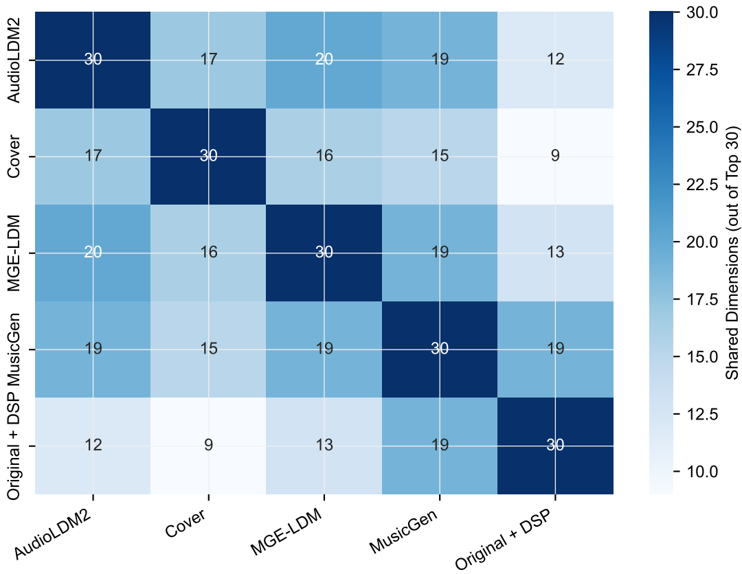
WEALY — Top-30 Dimension Overlap Between Categories All sources · Grouped by: Source
