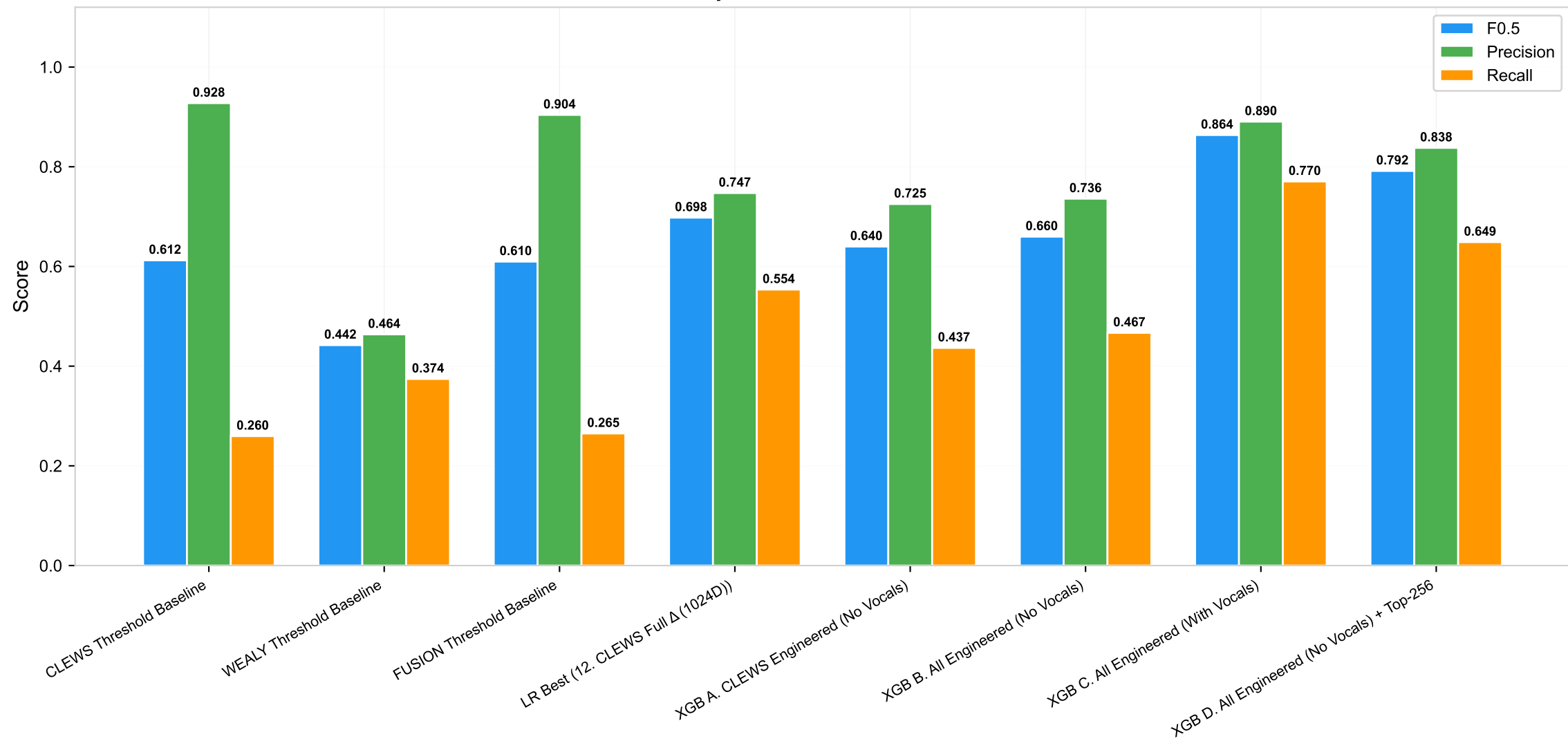
Final Classifier Comparison: Thresholds vs LR vs XGBoost
