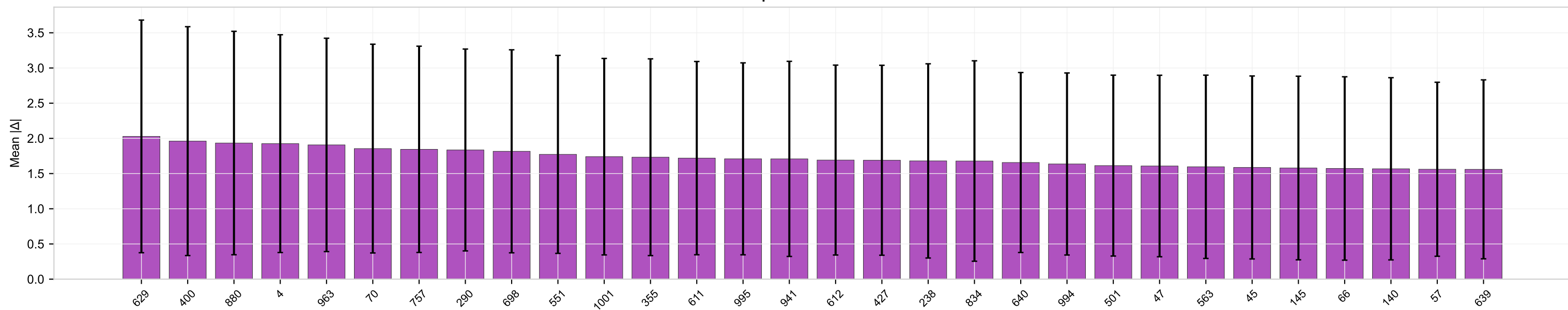
MusicGen — Top-30 Most Affected Dimensions
