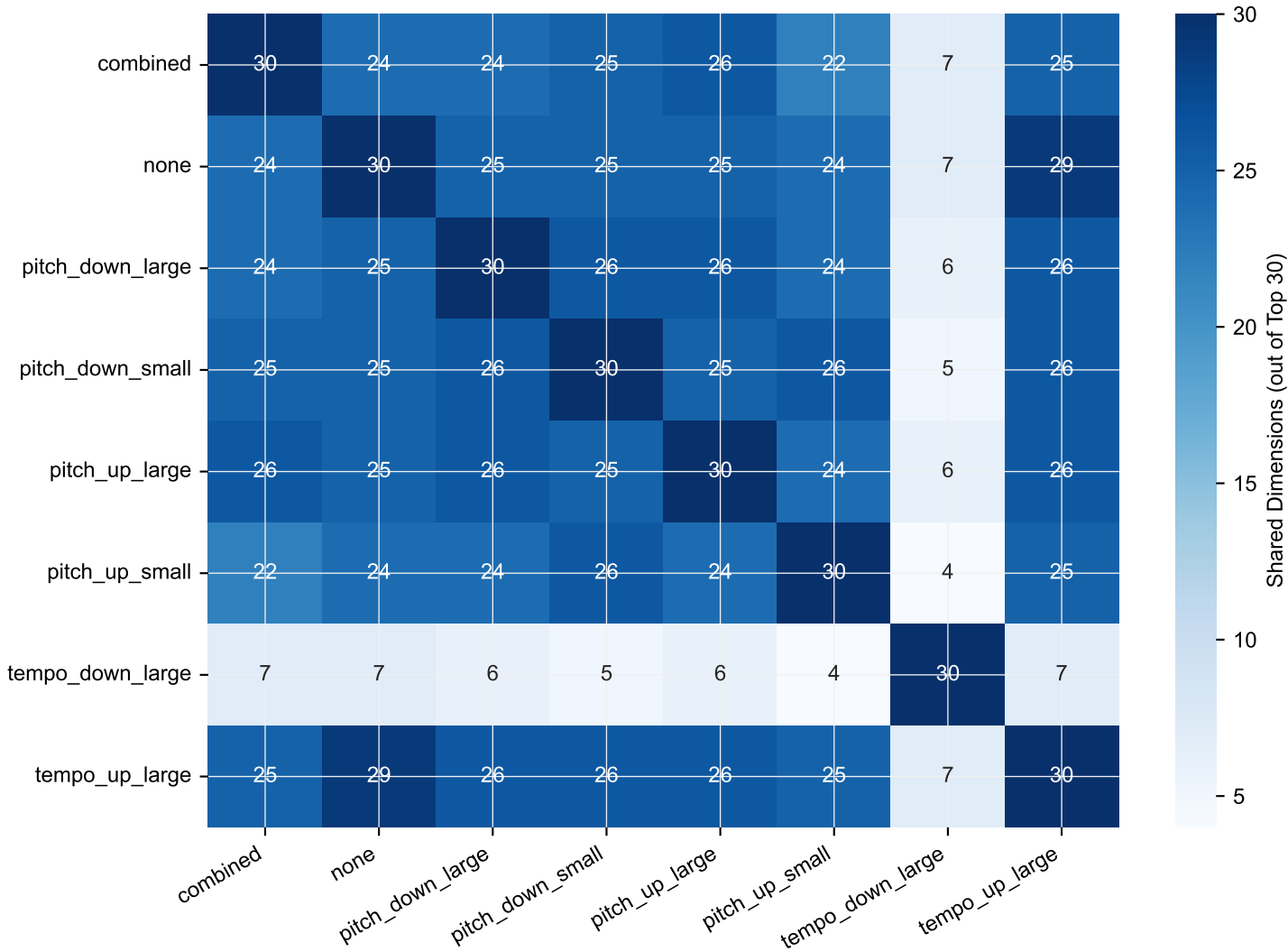
CLEWS — Top-30 Dimension Overlap Between Categories
