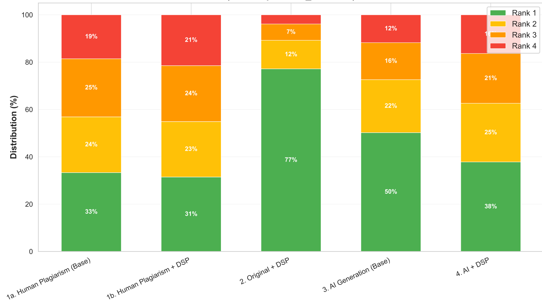
Rank Distribution of True Source — WEALY (metric: pearson_distance)
