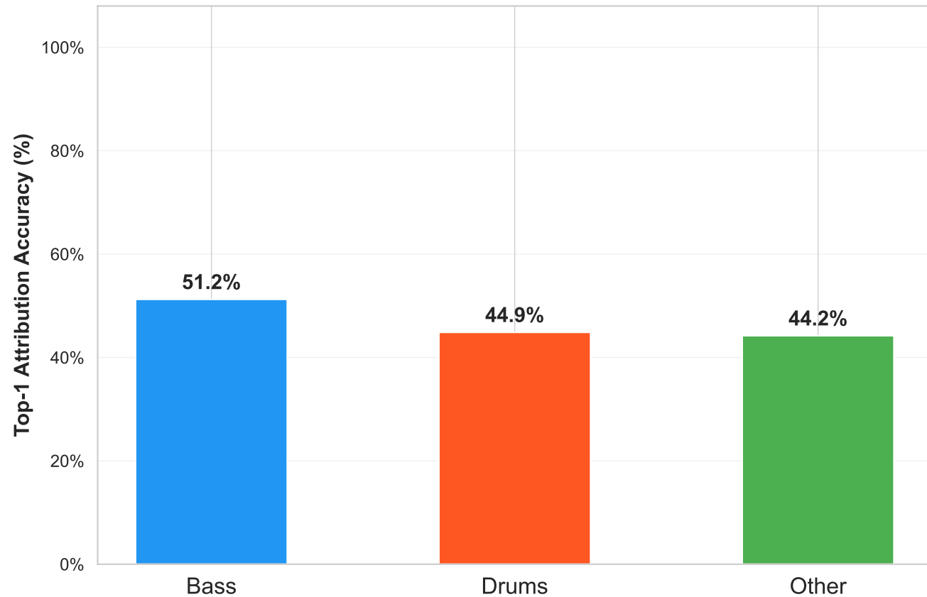
MGE-LDM Stem Attribution — WEALY (metric: pearson_distance, aggregated over all DSP variants)
