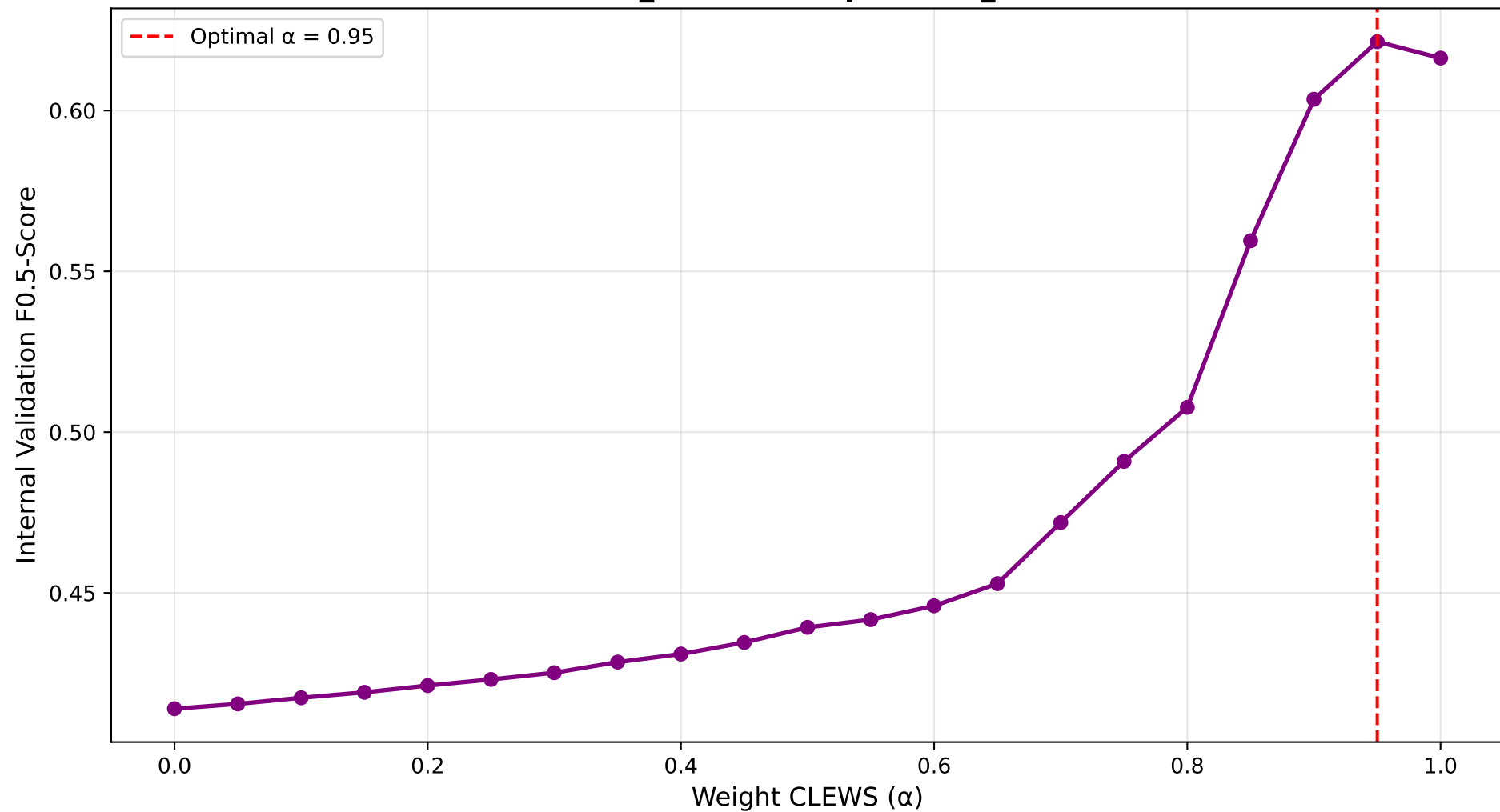
F0.5-Score vs Alpha (euclidean_distance & pearson_distance)
