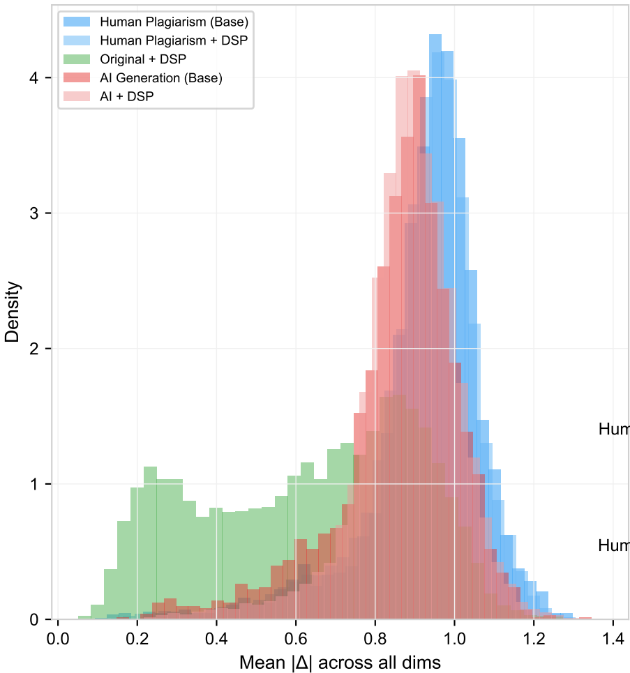
A) Overall Shift Distribution
