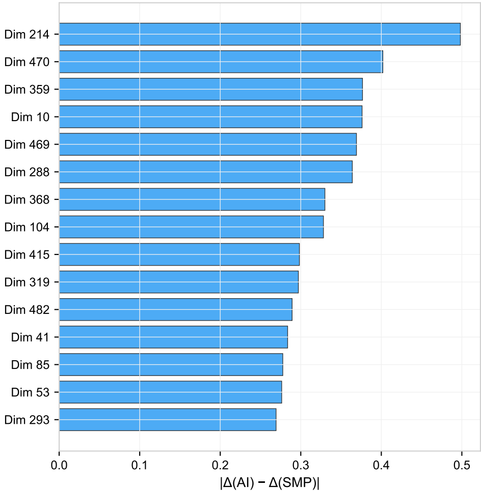
E) Top-15 Discriminating Dims (Red=AI, Blue=SMP)
