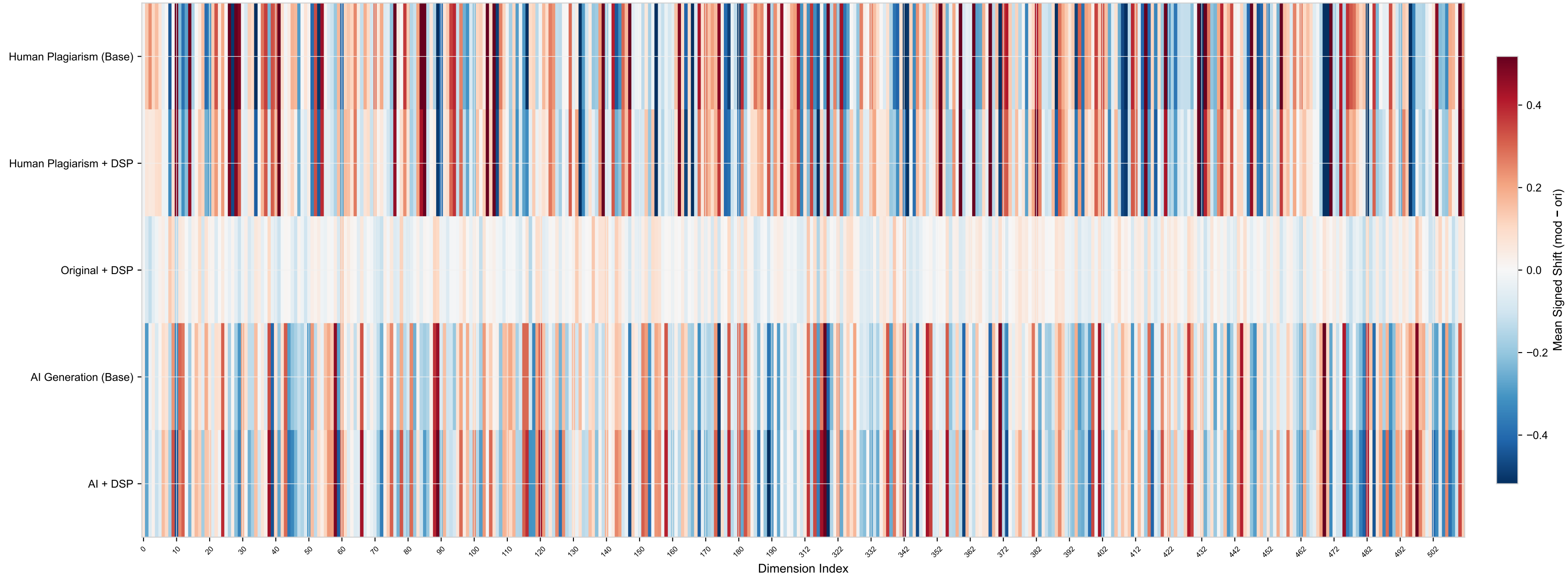
WEALY — Signed Mean Shift per Dimension (first 200 + last 200 of 512 dims)
