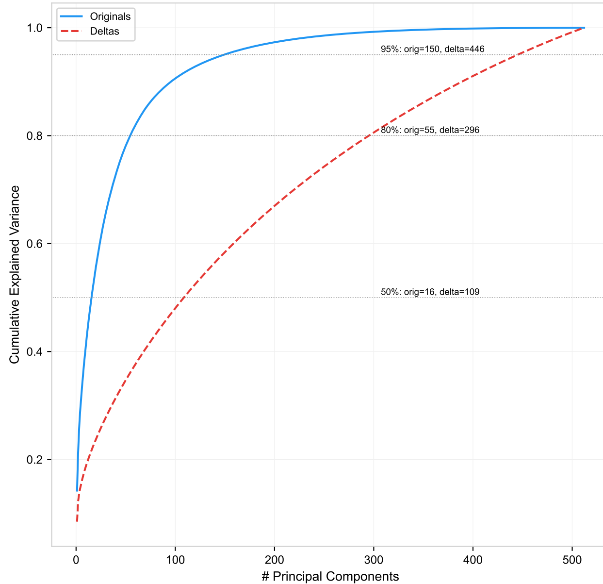
A) Cumulative Variance (Originals vs Deltas)
