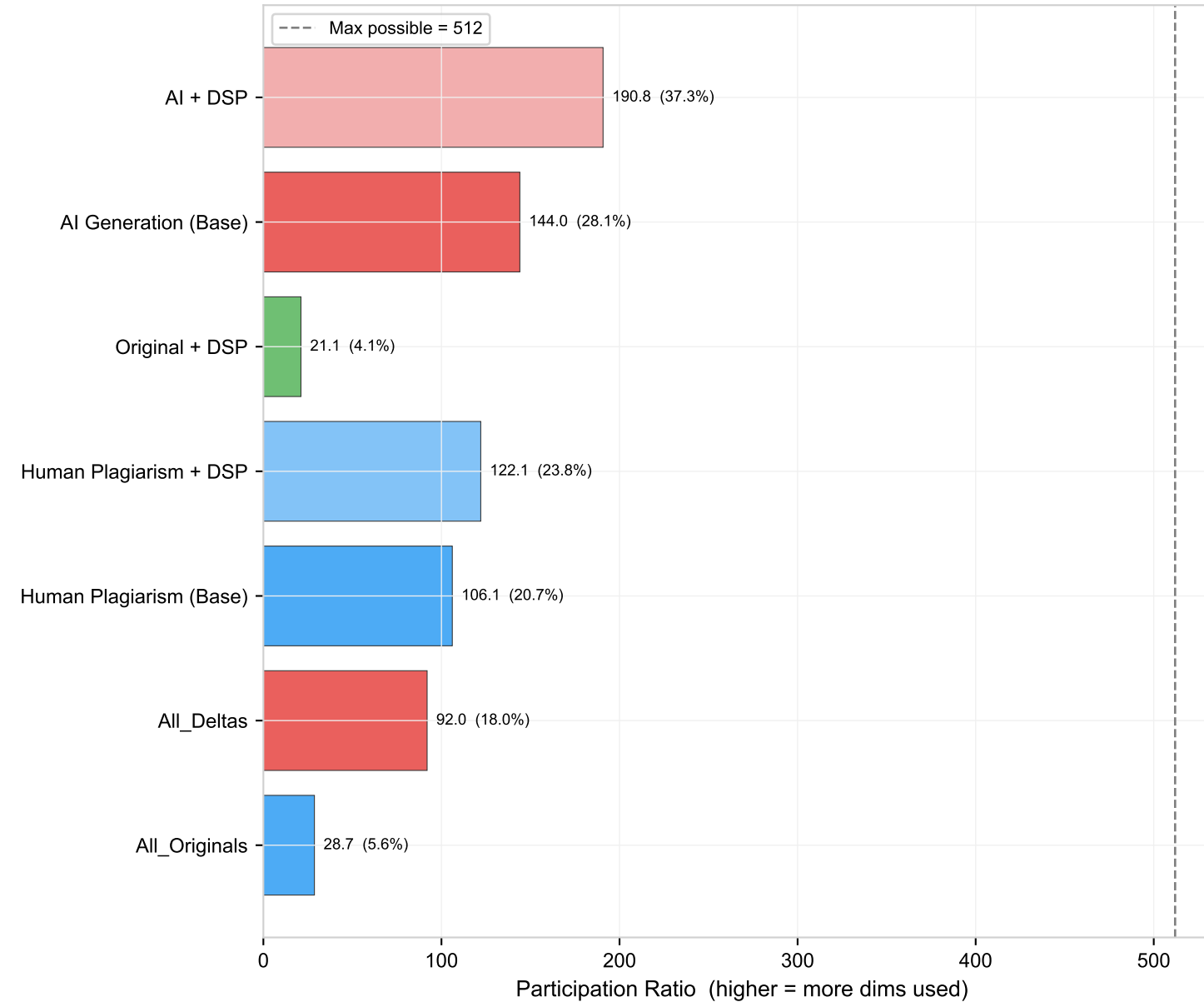
B) Effective Dimensionality per Subset
