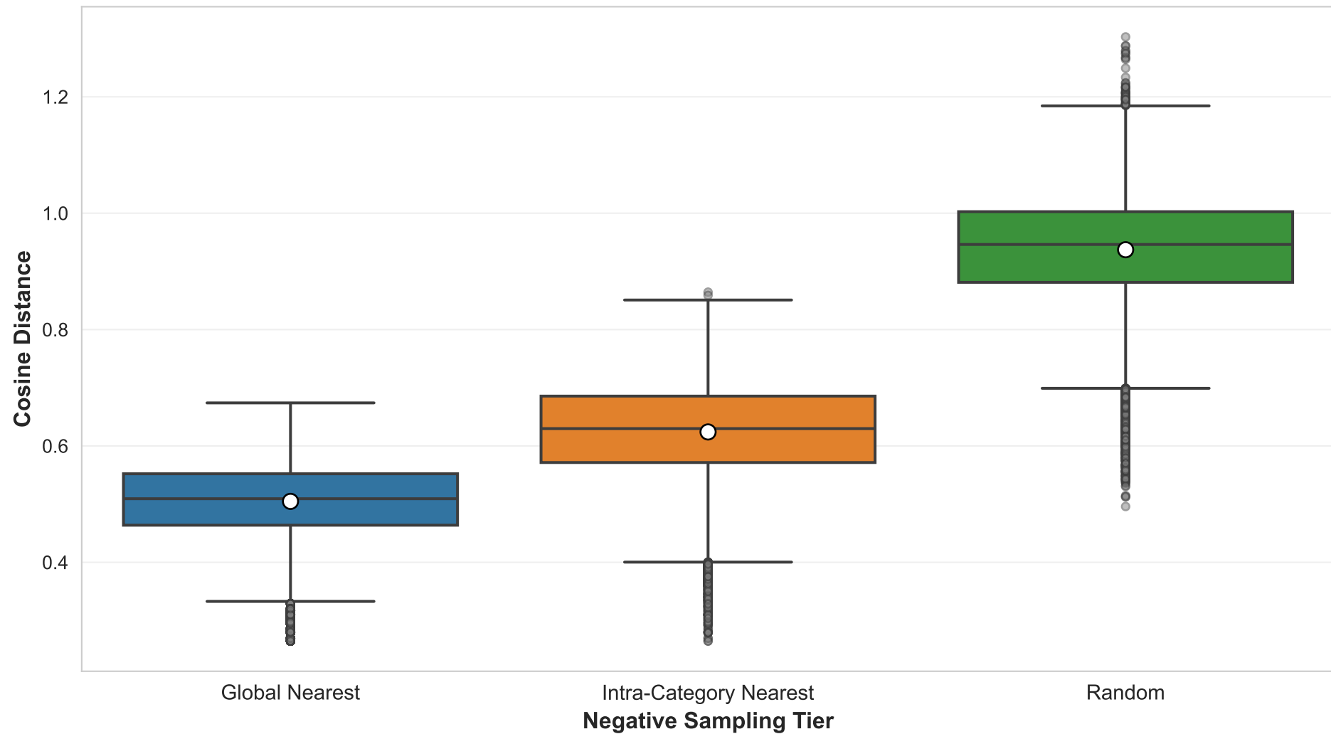
Distribution of Negative Tiers - CLEWS (Cosine Distance)
