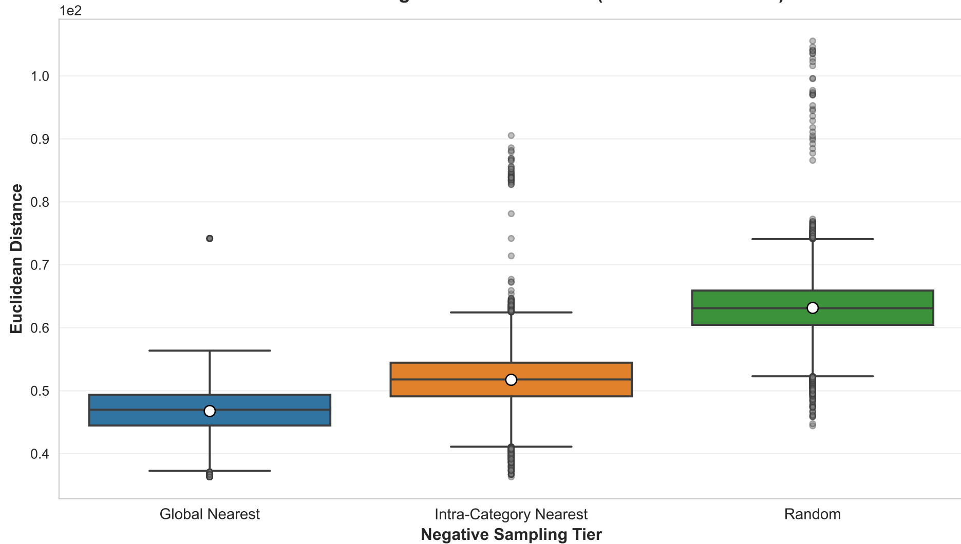
Distribution of Negative Tiers - CLEWS (Euclidean Distance)
