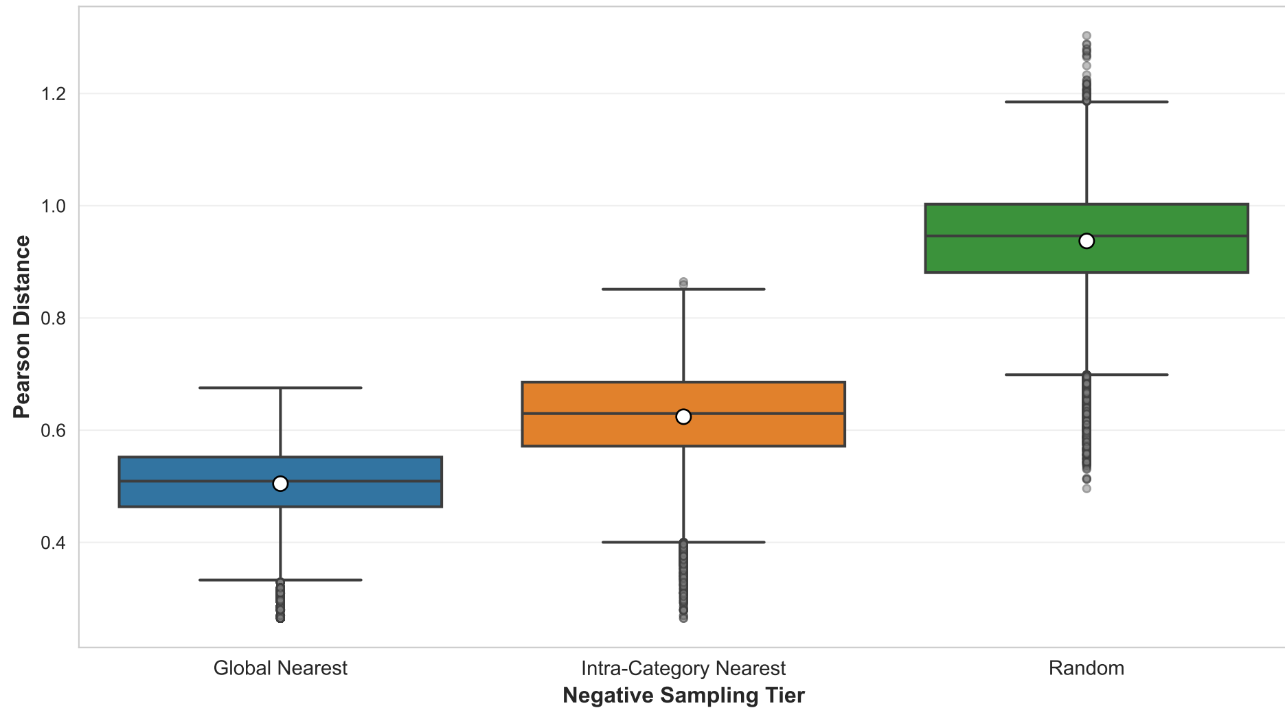
Distribution of Negative Tiers - CLEWS (Pearson Distance)
