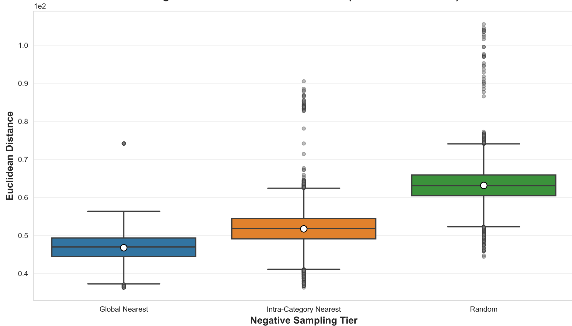
Negative Tier Distribution — CLEWS (Euclidean Distance)
