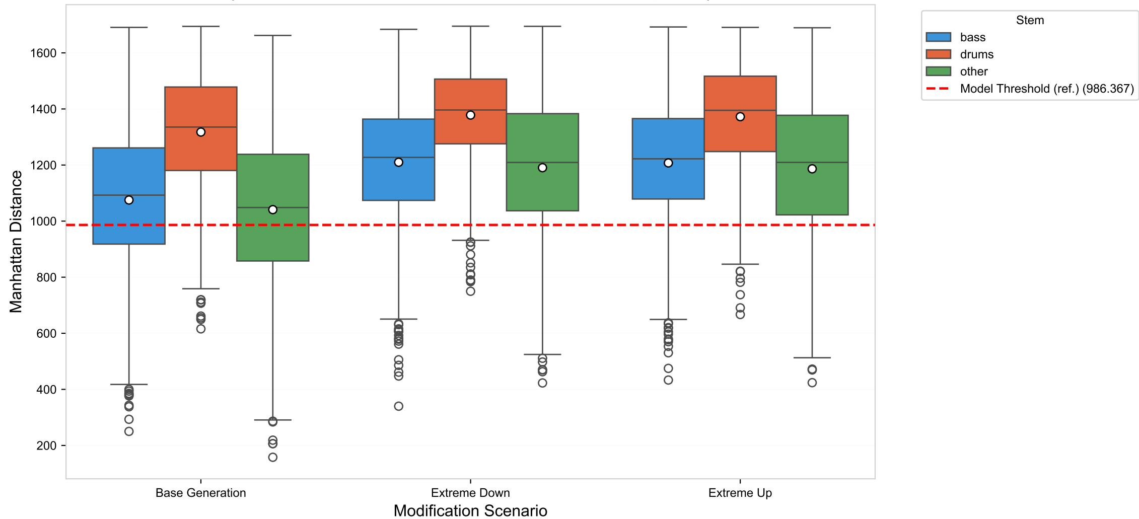
CLEWS — MGE-LDM Stem: Distance Under Extreme Stress (Threshold line = model-level reference, not stem-specific)
