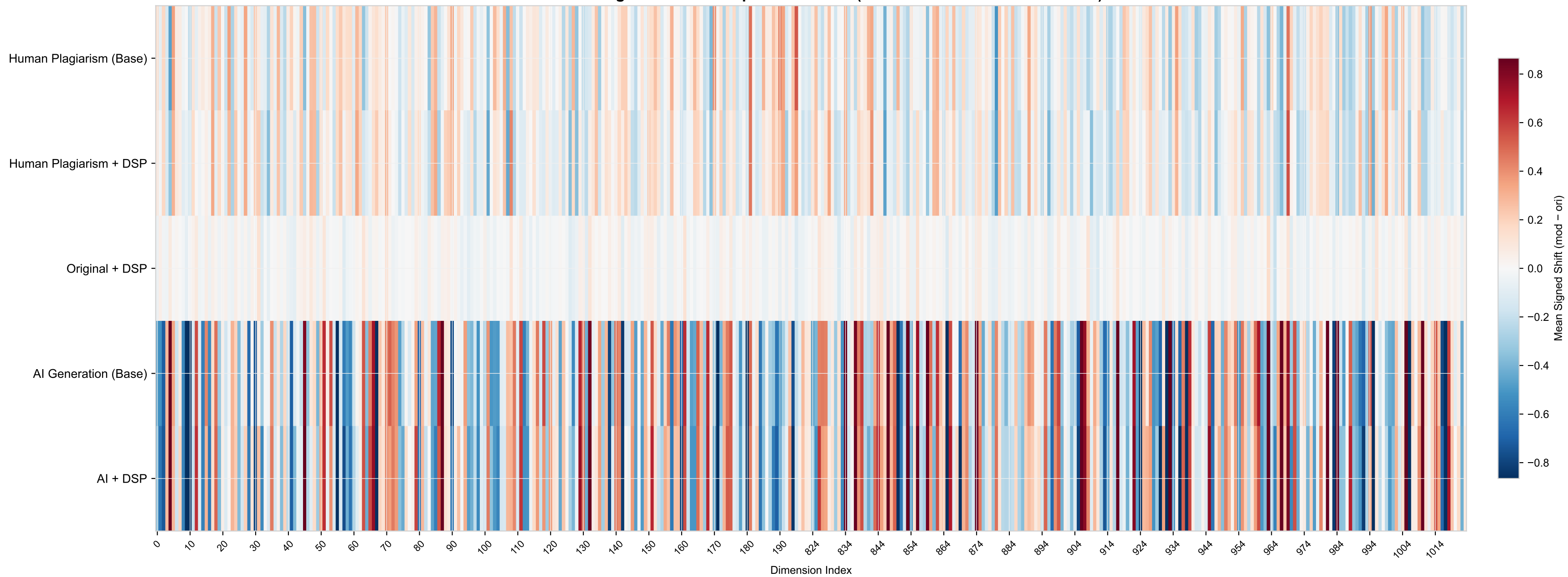
CLEWS — Signed Mean Shift per Dimension (first 200 + last 200 of 1024 dims)
