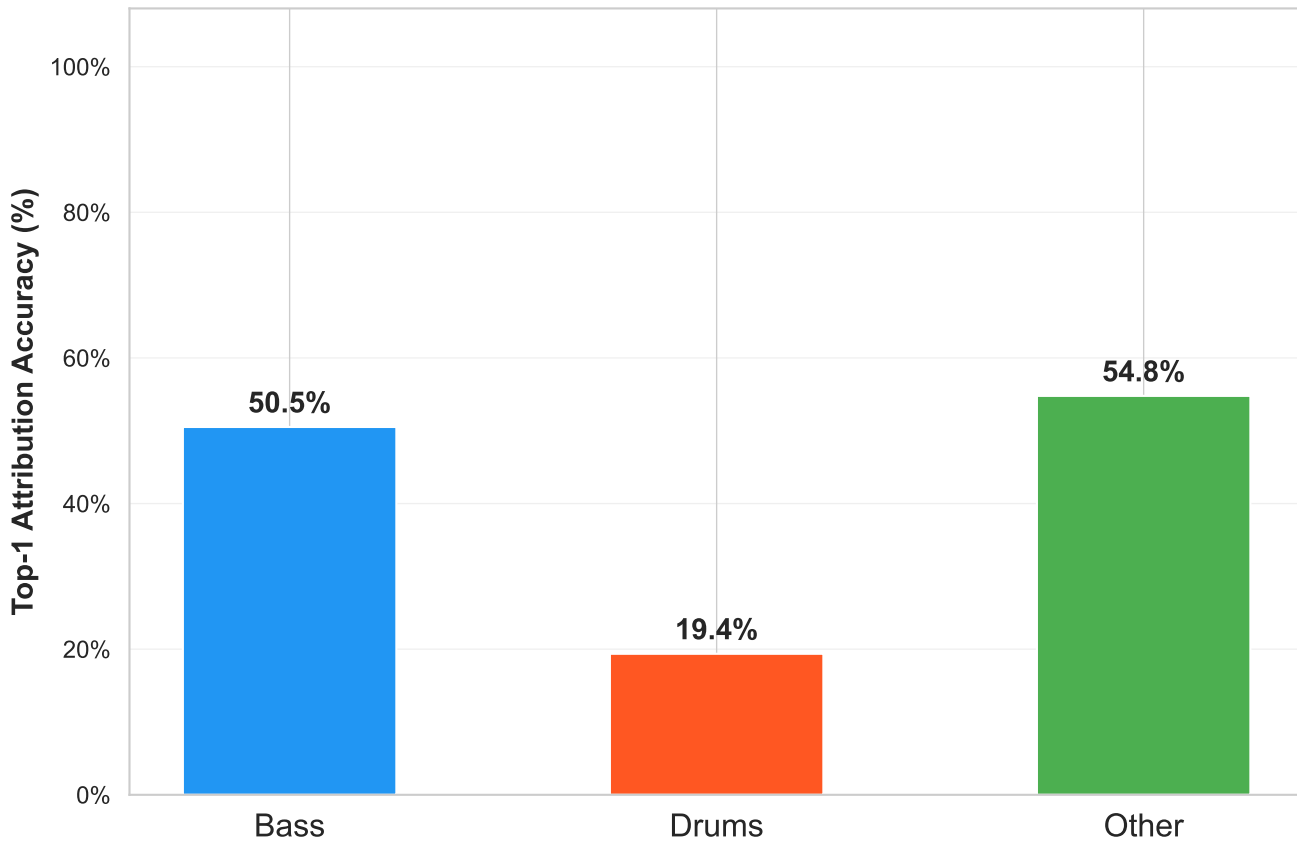
MGE-LDM Stem Attribution — CLEWS (metric: manhattan_distance, aggregated over all DSP variants)
