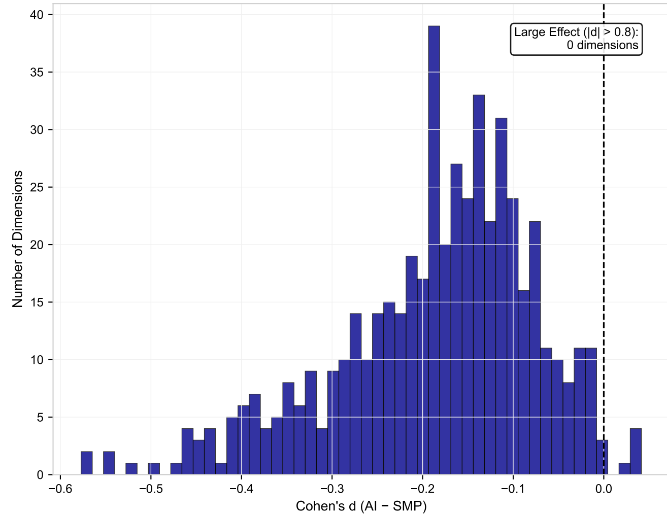
B) Effect Size Distribution (Separability)
