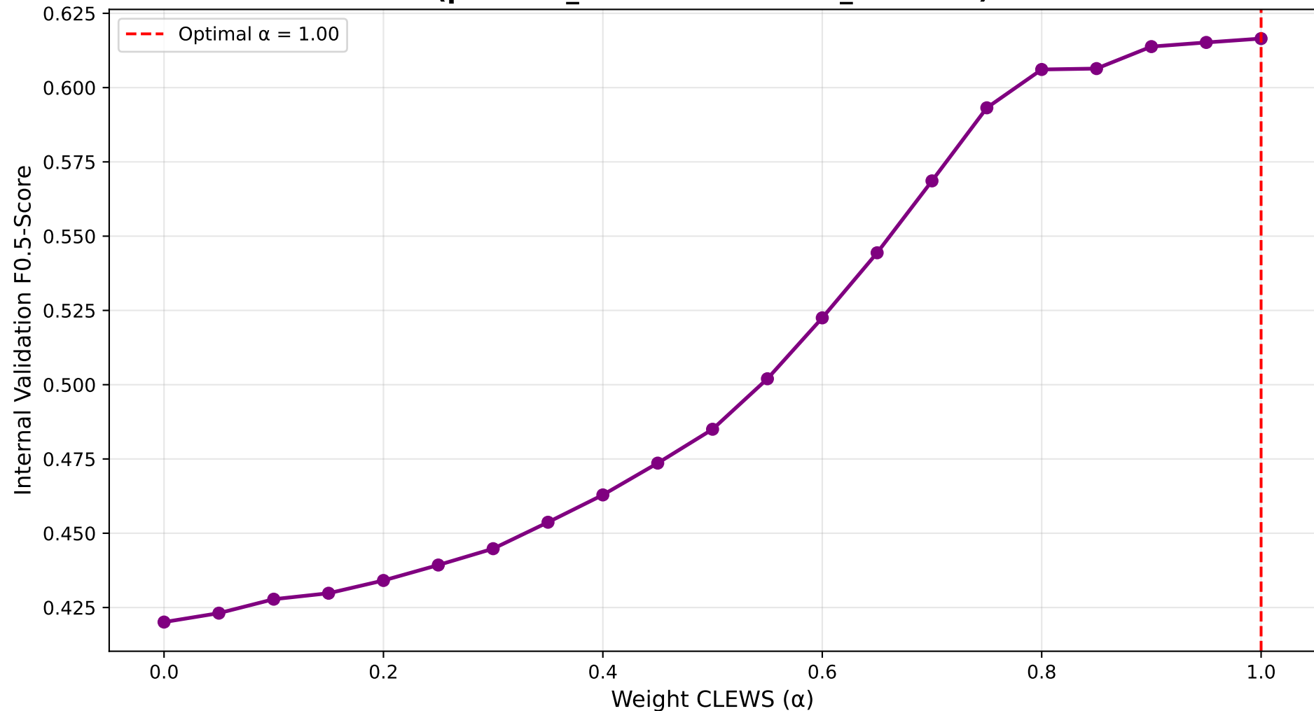
F0.5-Score vs Alpha (pearson_distance & cosine_distance)
