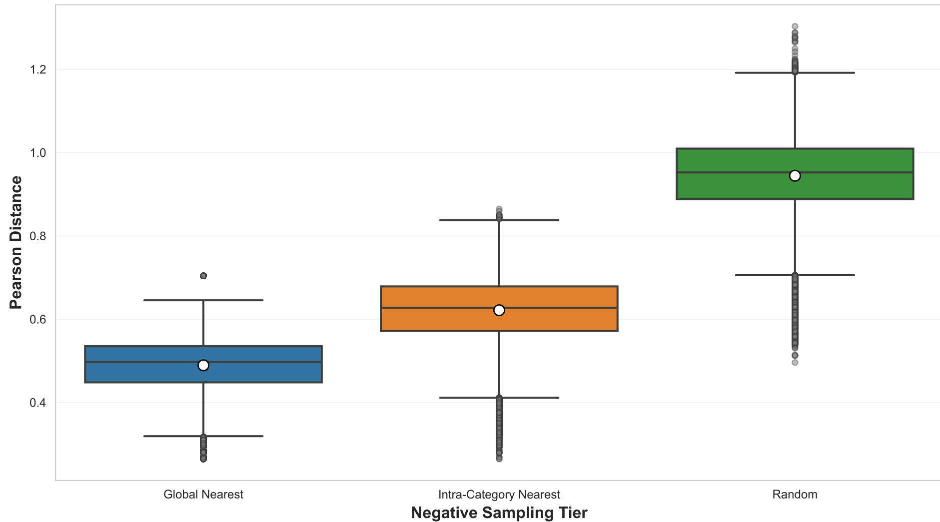
Negative Tier Distribution — CLEWS (Pearson Distance)
