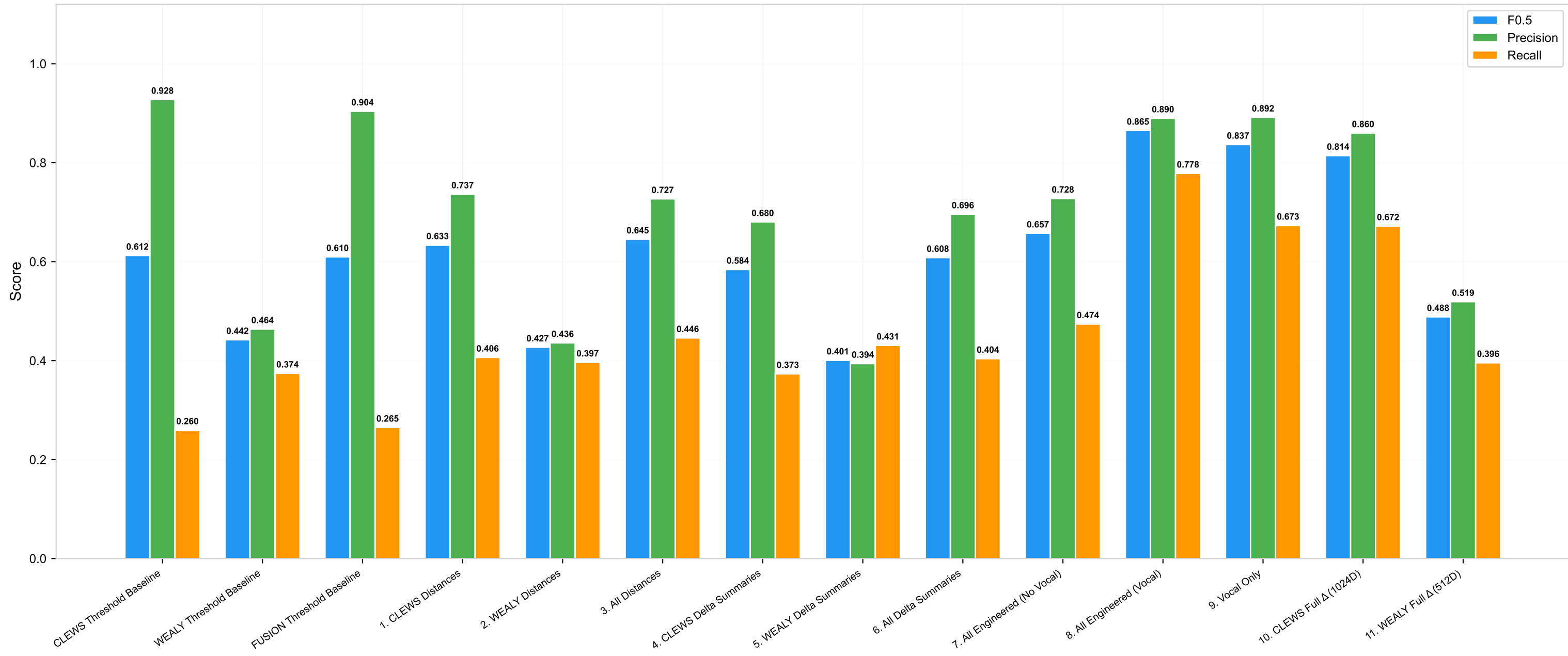
Feature Ablation: Classification Performance (XGBoost Classifier)
