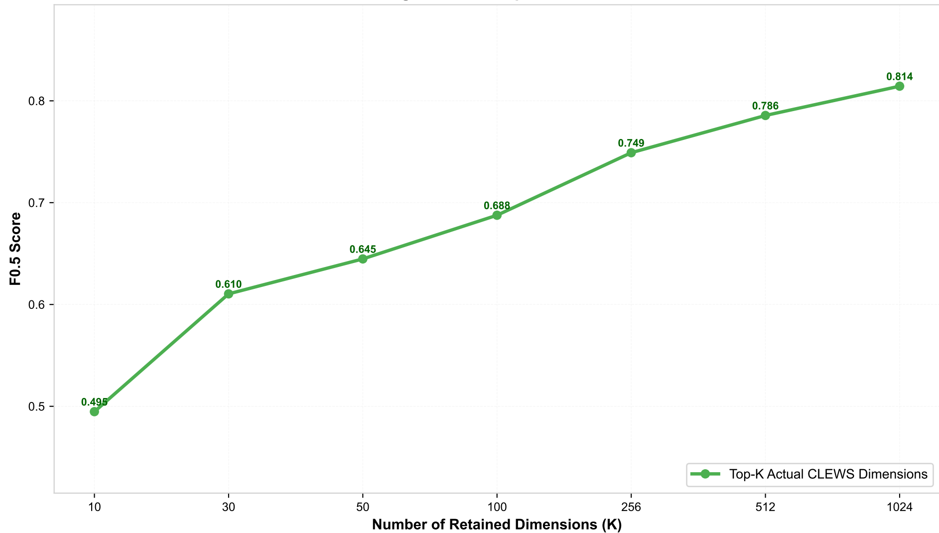
Classification Convergence with Top-K Actual CLEWS Dimensions
