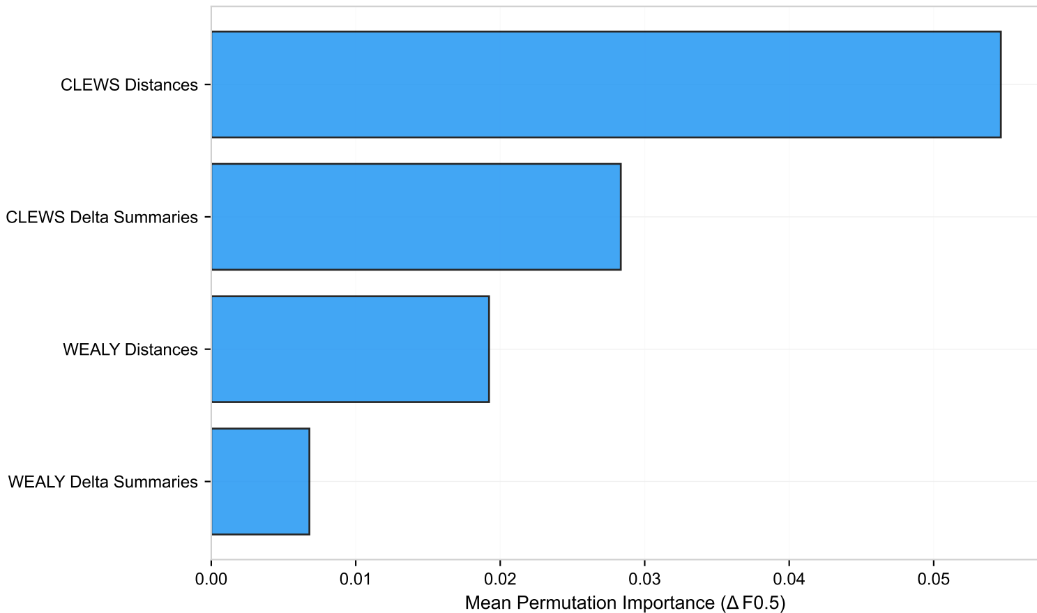
engineered_no_vocals — Feature Family Importance
