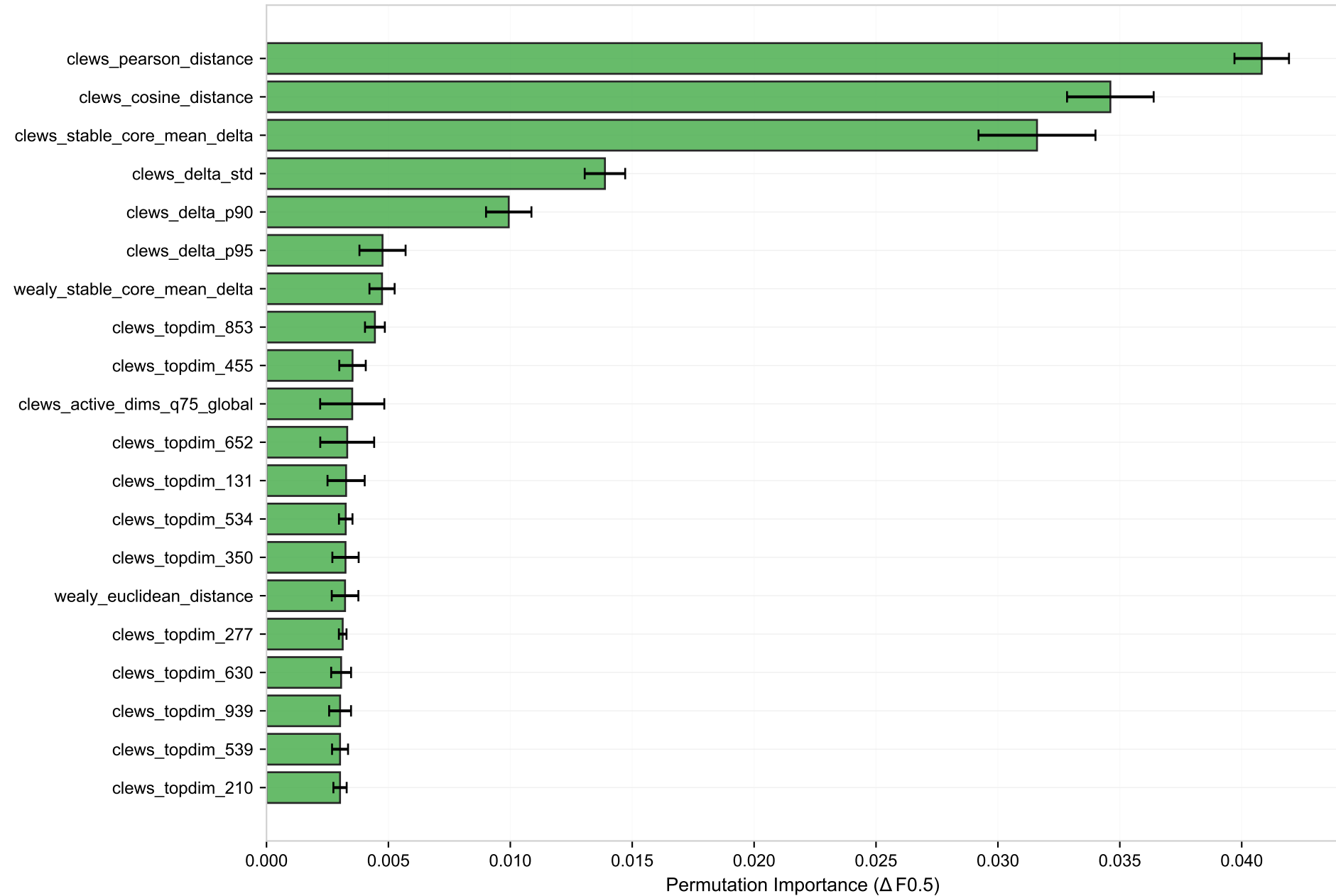
hybrid_top512 — Top-20 Feature Importances
