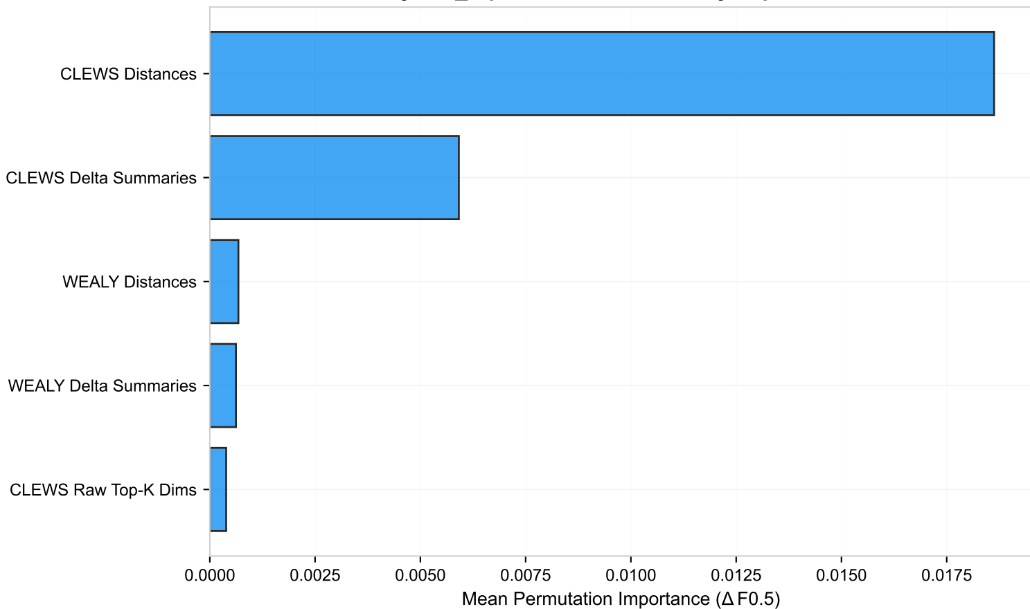
hybrid_top512 — Feature Family Importance
