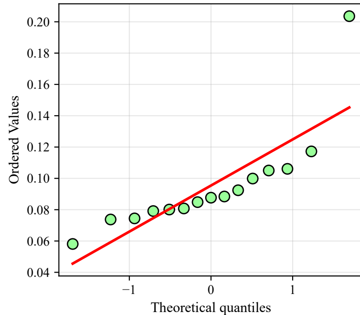
SC-PINN Shapiro-Wilk p=0.0004
