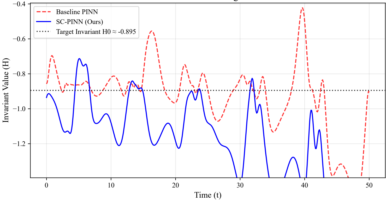
Invariant Evolution over Integration Horizon
