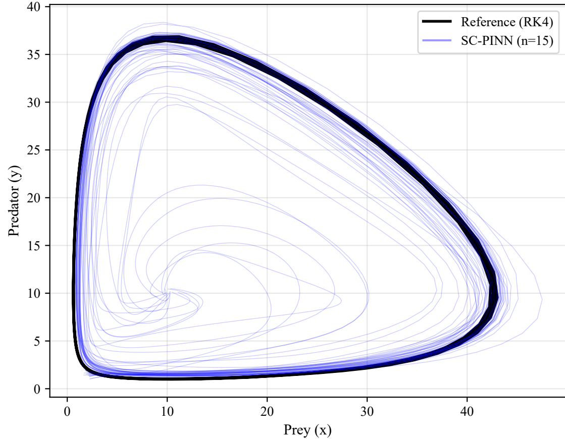
SC-PINN: Phase-Space Variability
