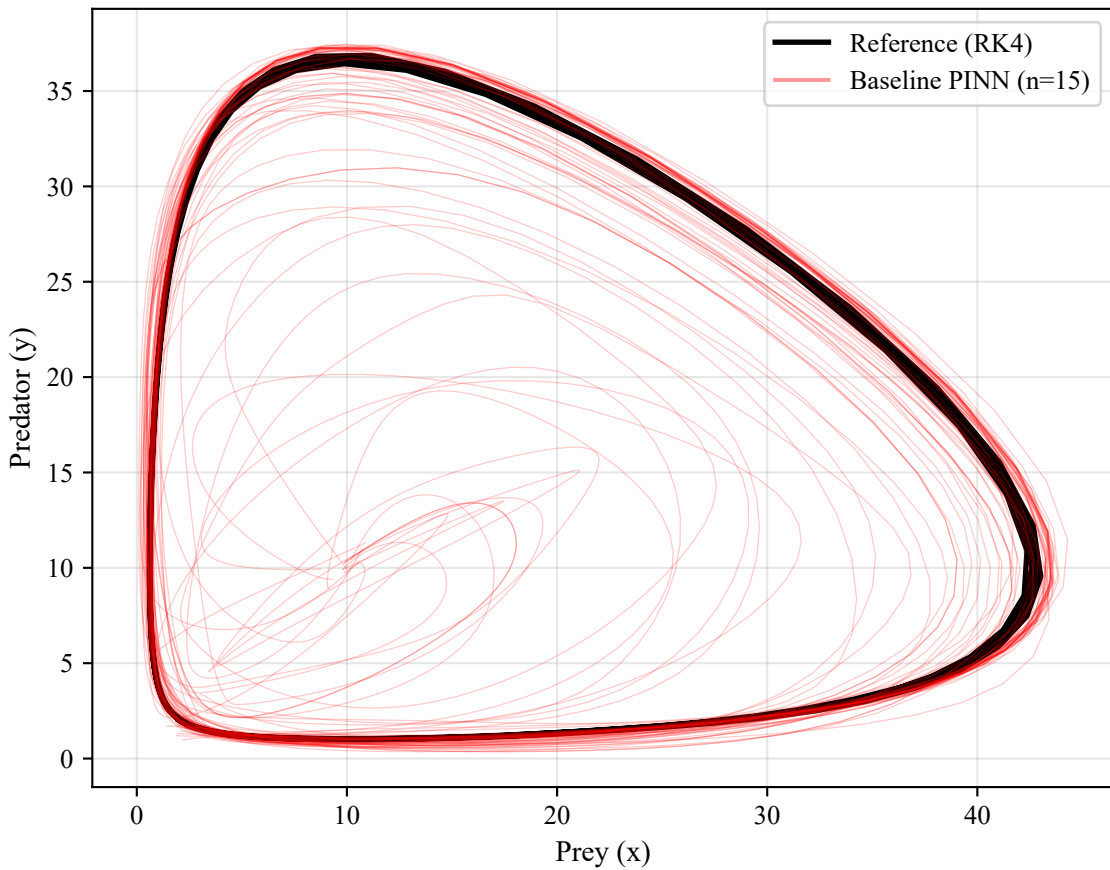
Baseline PINN: Phase-Space Variability
