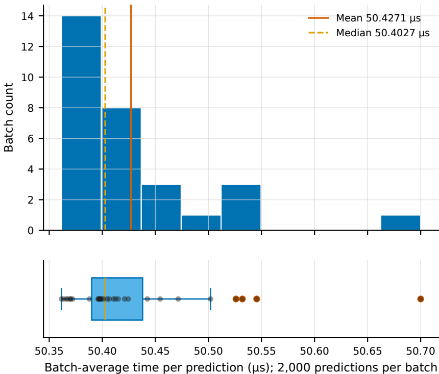
ESP8266 model-kernel timing across 30 batch averages
