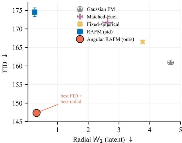
DC-AE ImageNette: FID vs radial calibration
