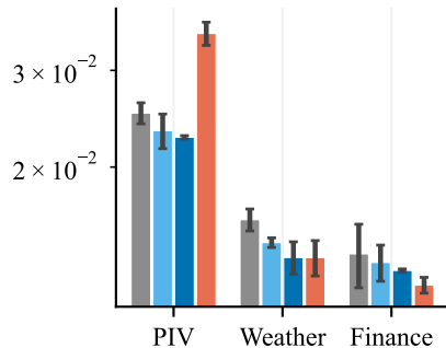
Angular SW
