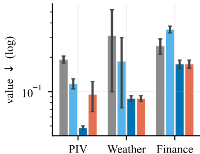
Radial W_1
