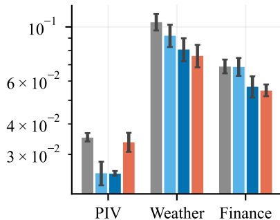
Sliced W_1
