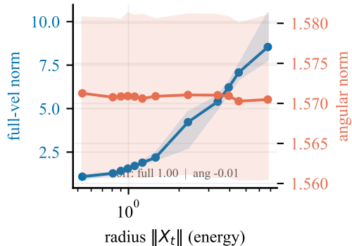
Target norm vs radius
