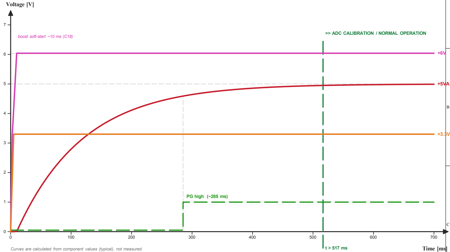
Curves are calculated from component values (typical), not measured.
